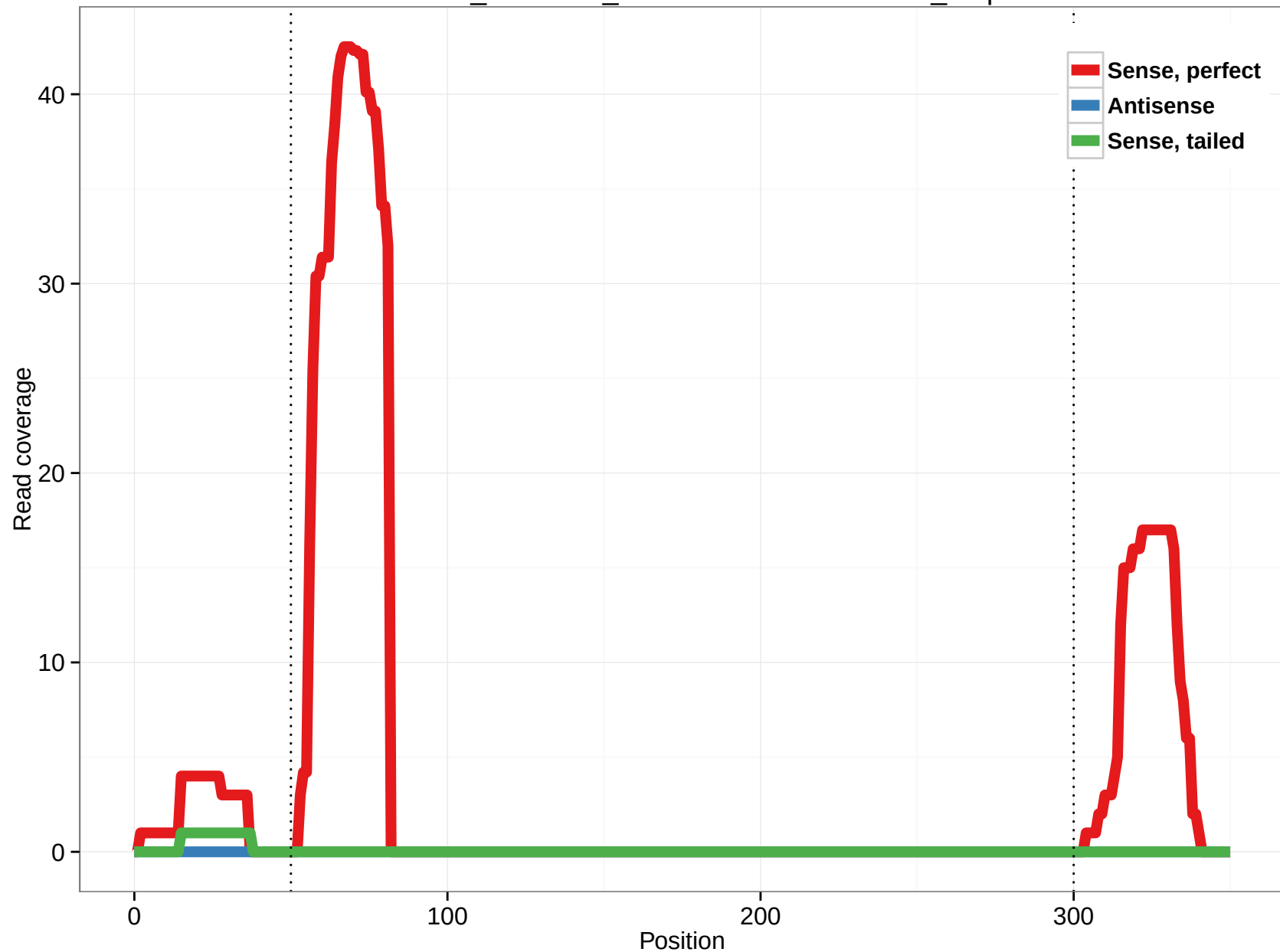
ornAna1_ensGene_ENSOANT00000029144_1.3p
