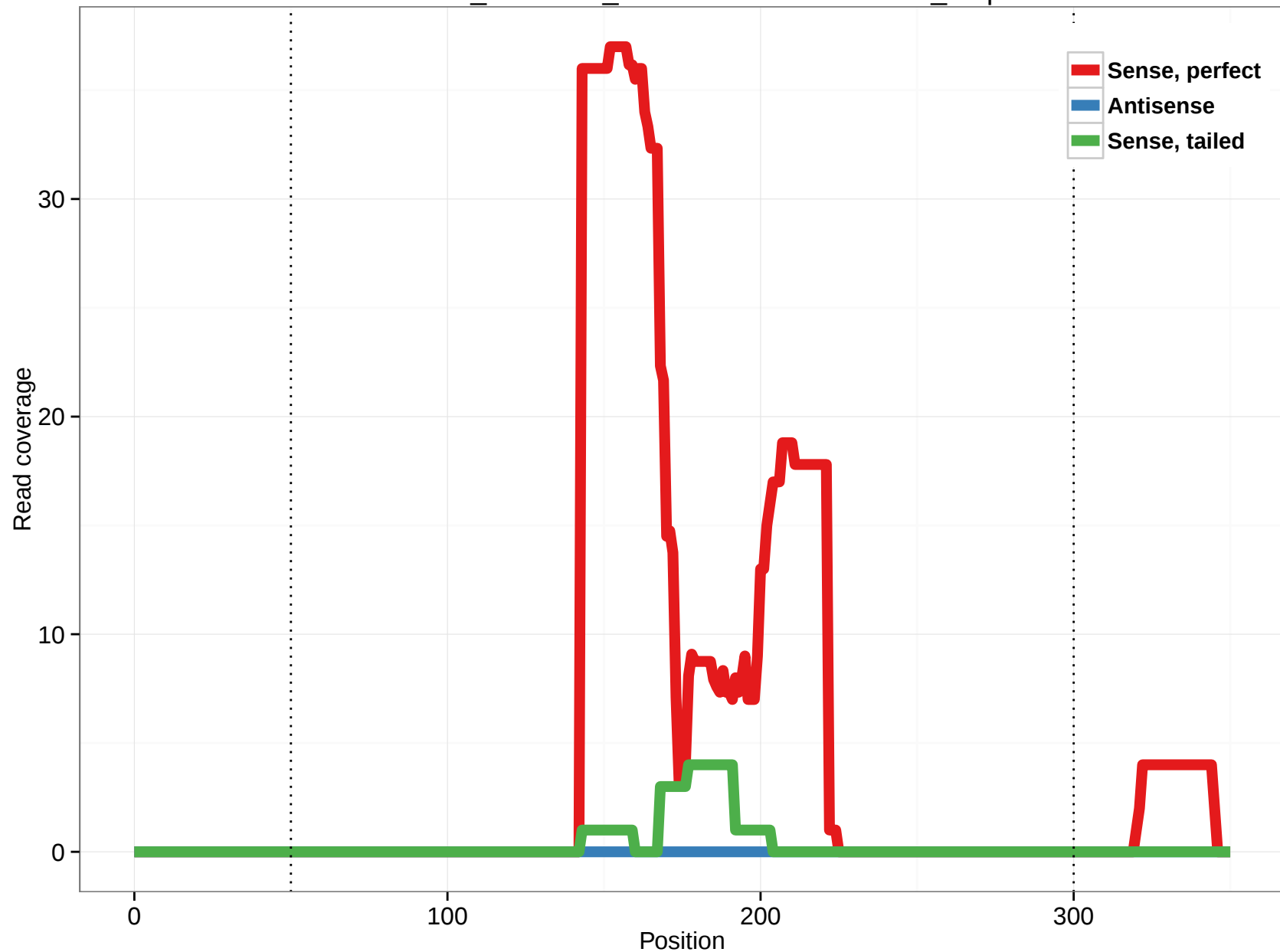
ornAna1_ensGene_ENSOANT00000029065_2.3p
