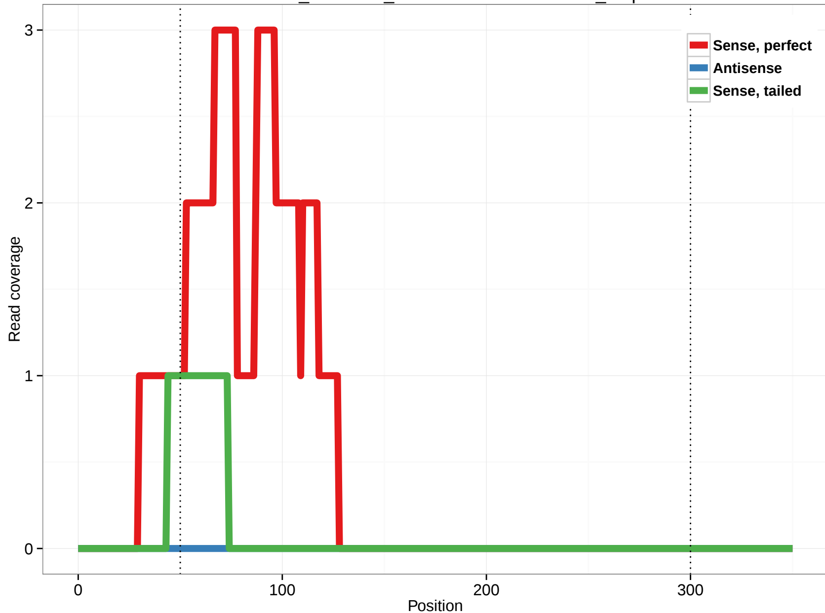
ornAna1_ensGene_ENSOANT00000029003_4.5p
