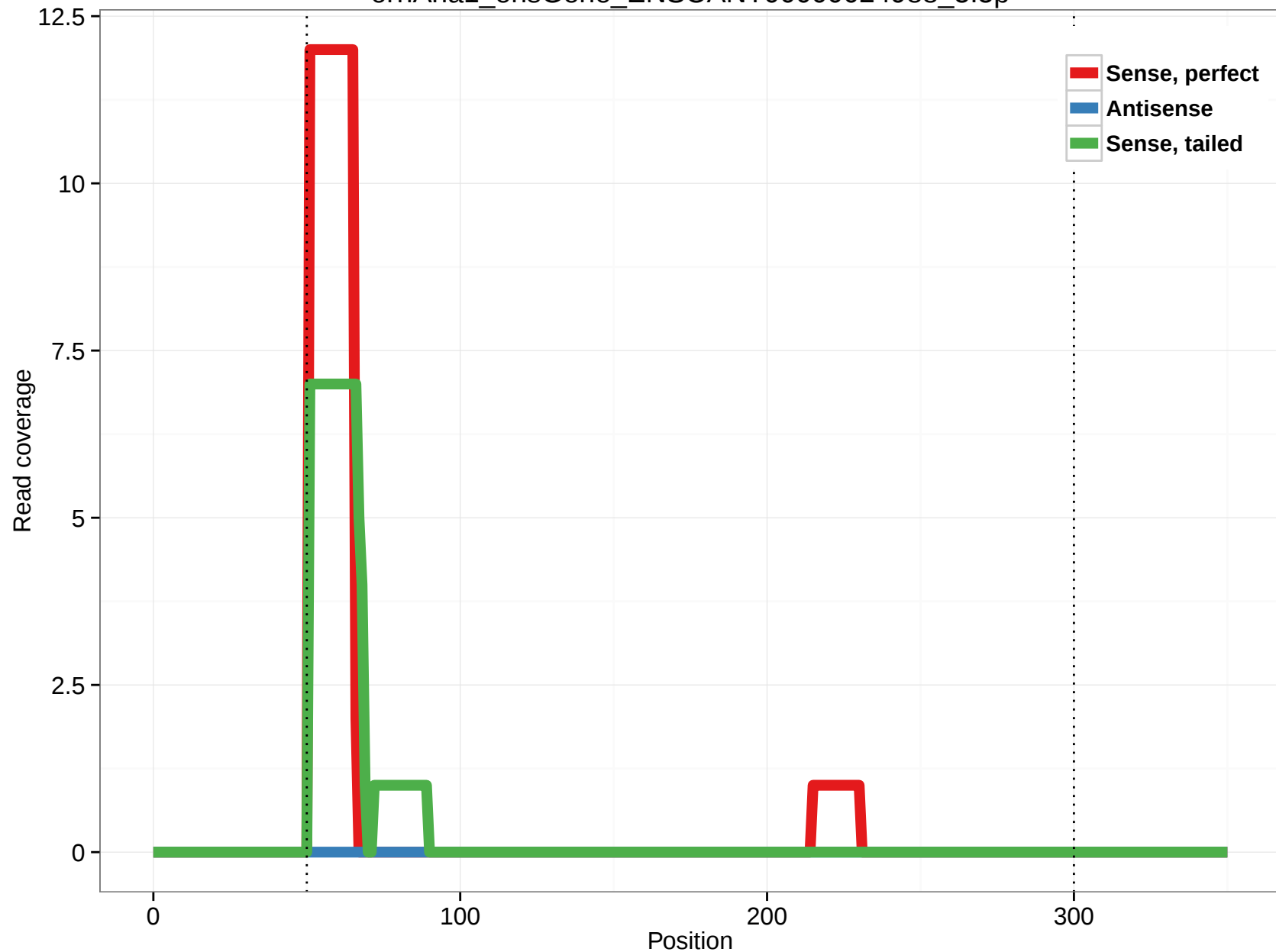
ornAna1_ensGene_ENSOANT00000024988_5.5p
