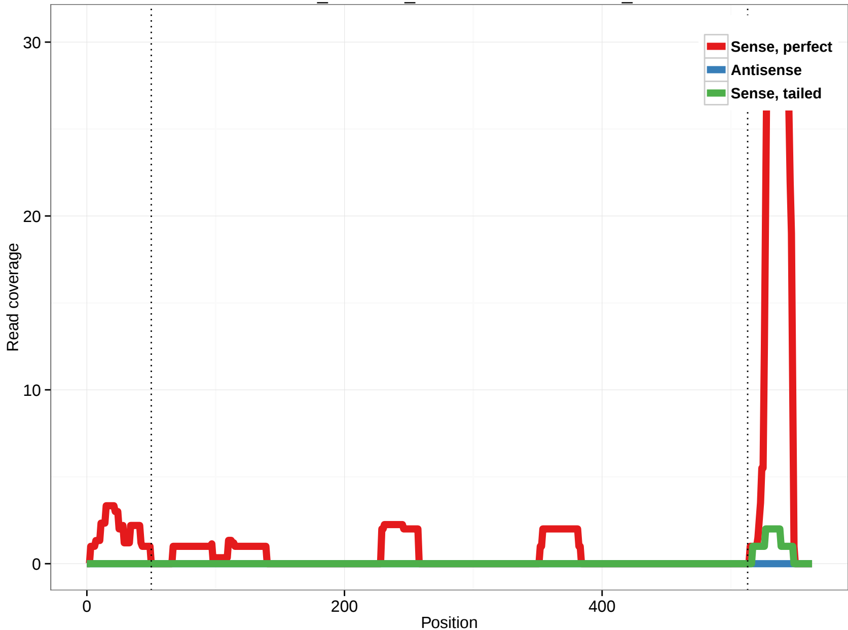
ornAna1_ensGene_ENSOANT00000024957_13
