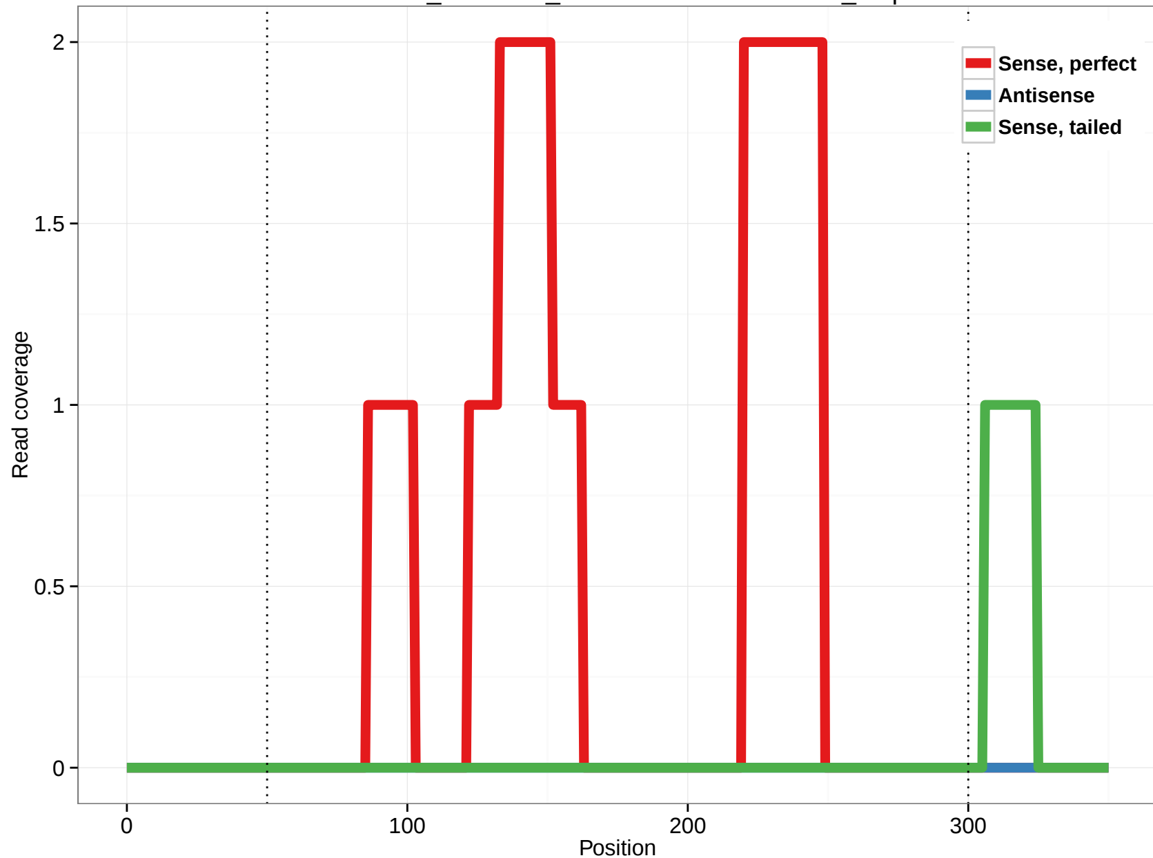
ornAna1_ensGene_ENSOANT00000024937_9.3p
