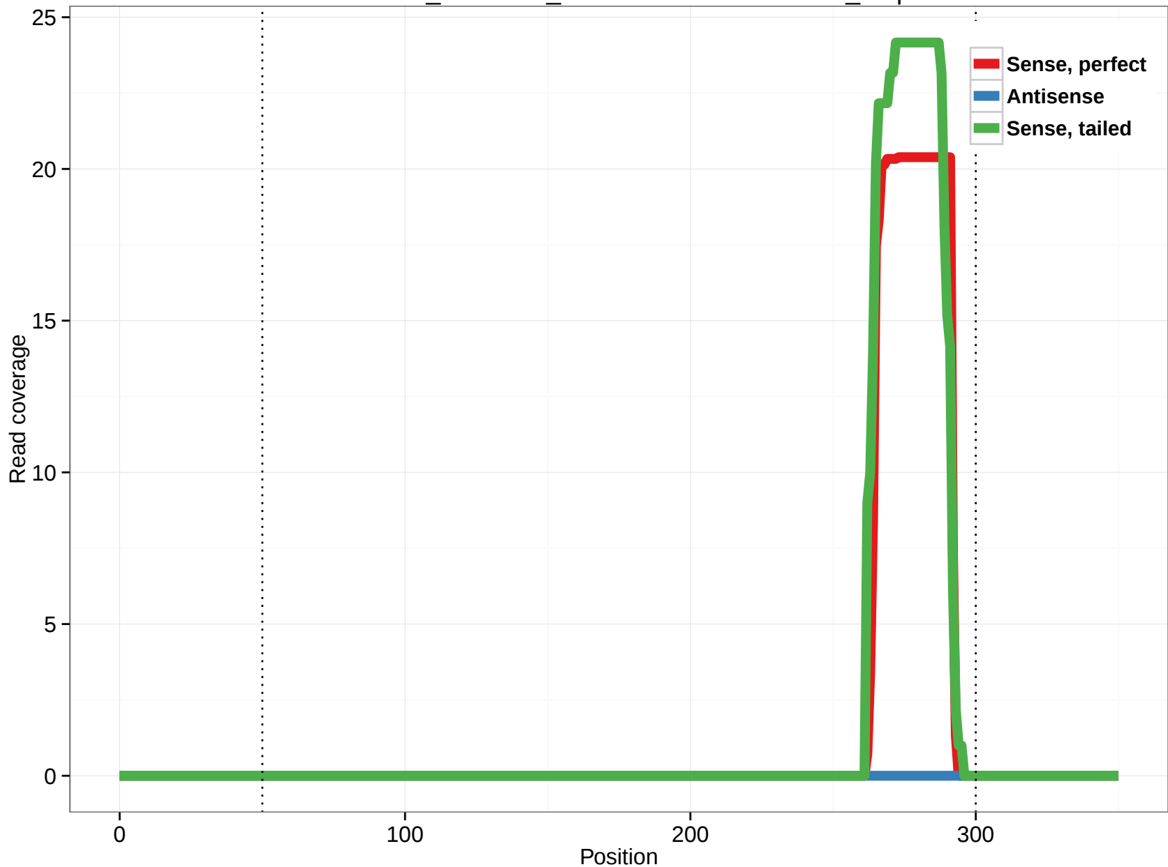
ornAna1_ensGene_ENSOANT00000024918_2.5p
