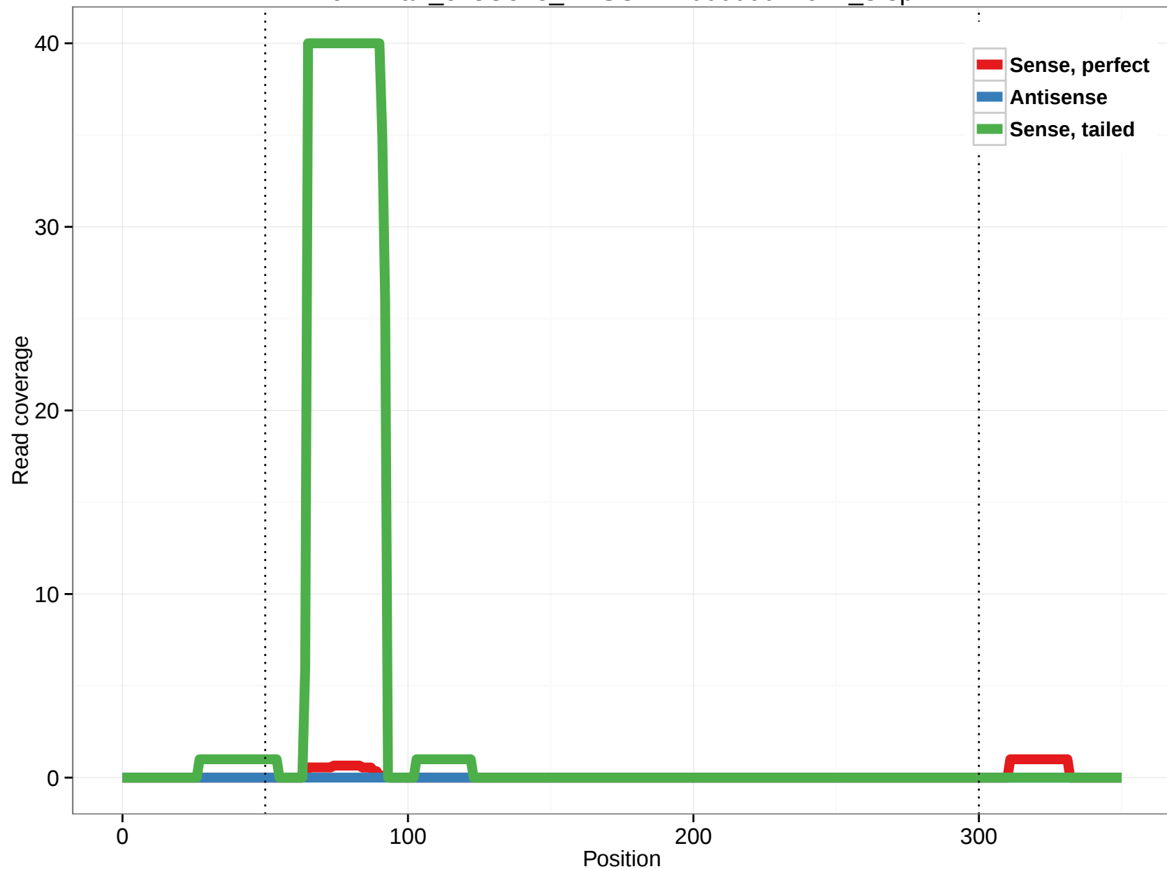
ornAna1_ensGene_ENSOANT00000024912_3.3p
