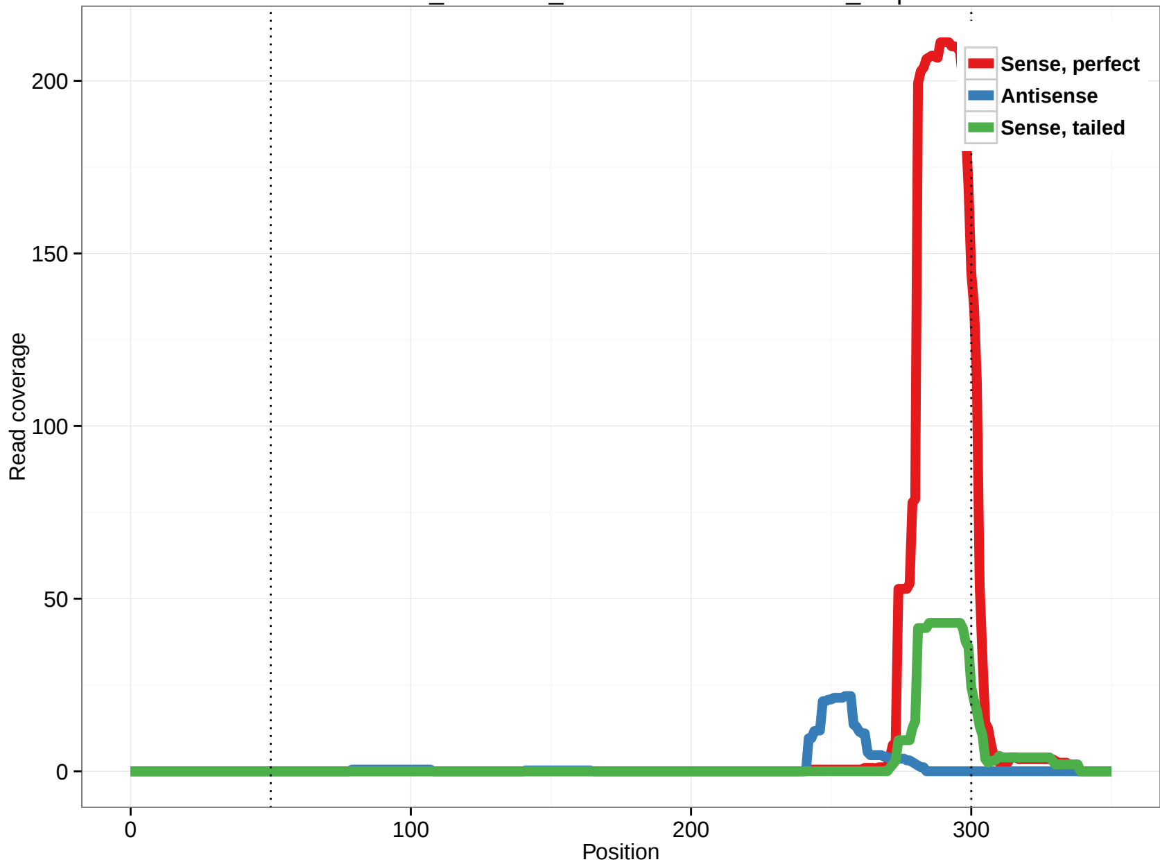
ornAna1_ensGene_ENSOANT00000024817_5.5p
