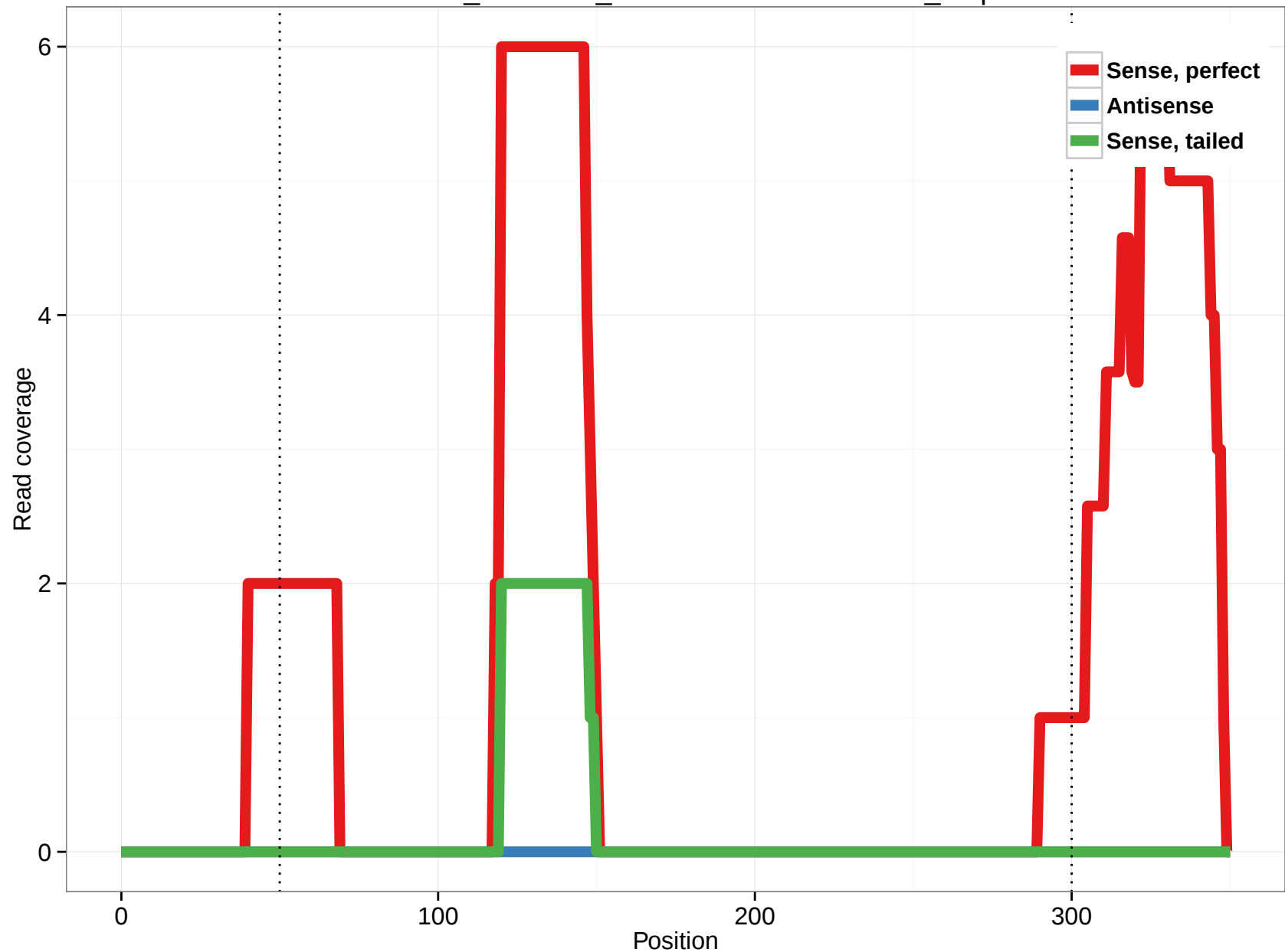
ornAna1_ensGene_ENSOANT00000024816_2.3p
