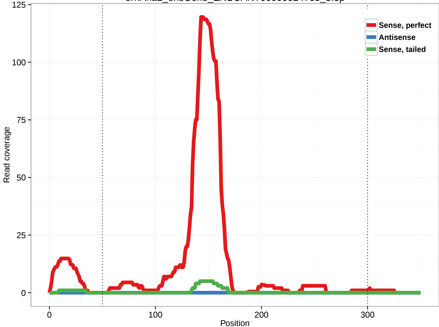
ornAna1_ensGene_ENSOANT00000024765_3.5p
