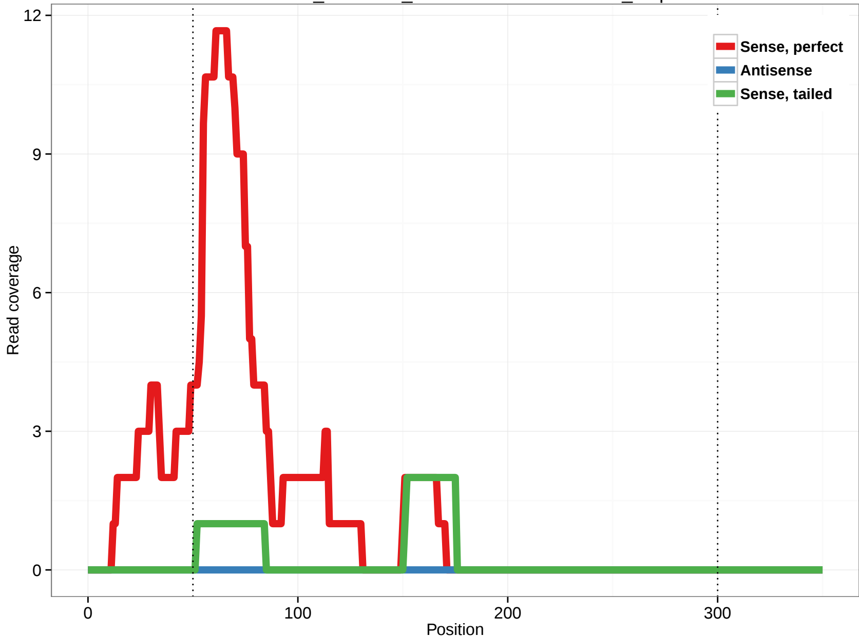
ornAna1_ensGene_ENSOANT00000024760_0.5p
