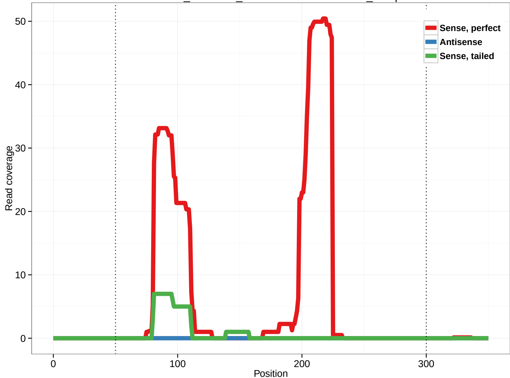
ornAna1_ensGene_ENSOANT00000024749_24.3p
