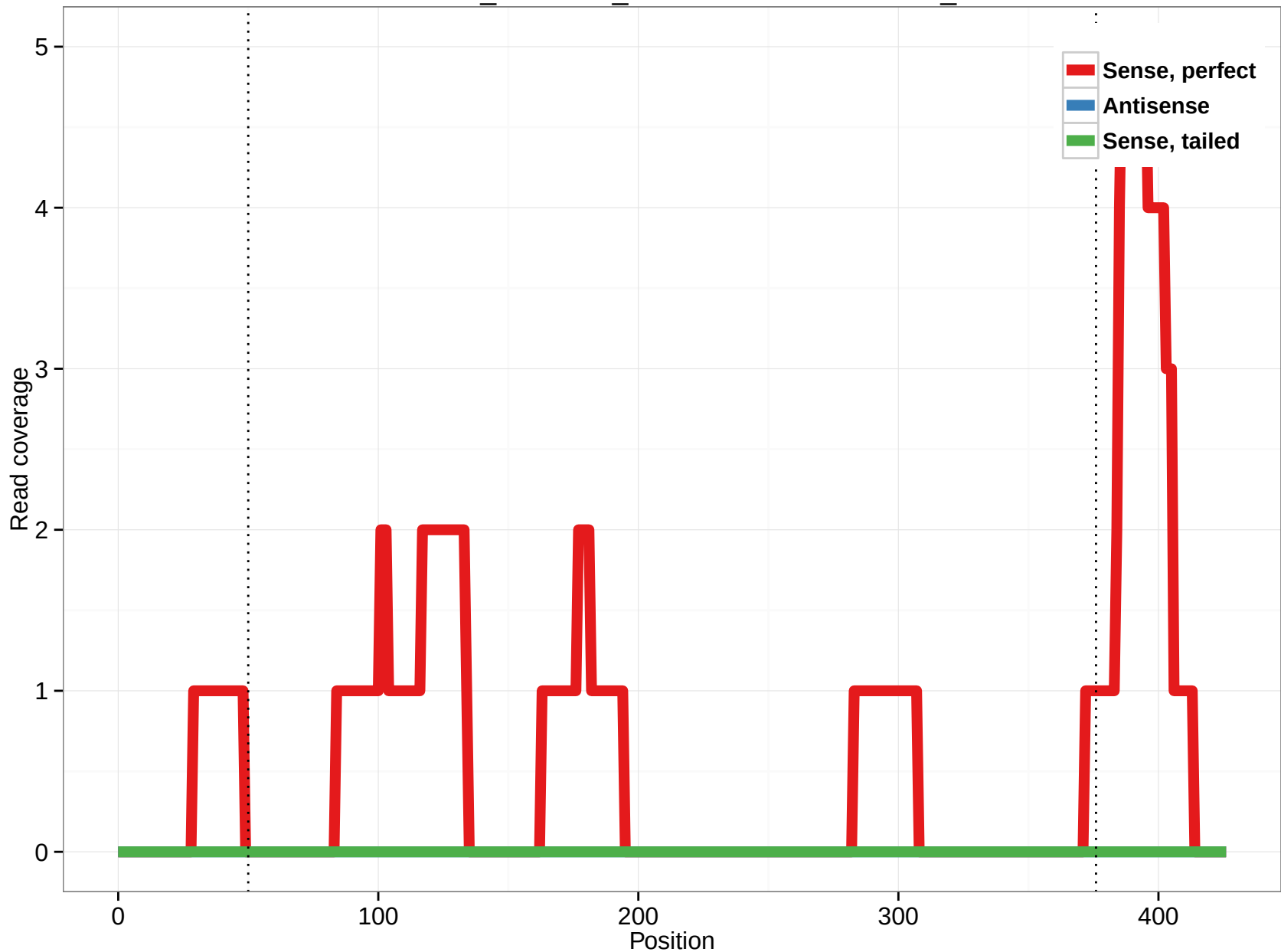
ornAna1_ensGene_ENSOANT00000024718_7
