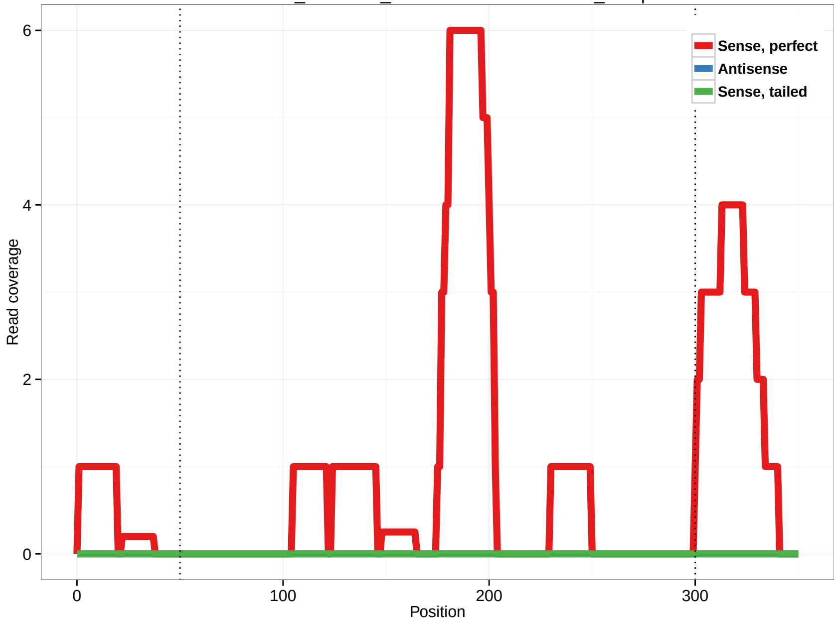
ornAna1_ensGene_ENSOANT00000024624_18.3p
