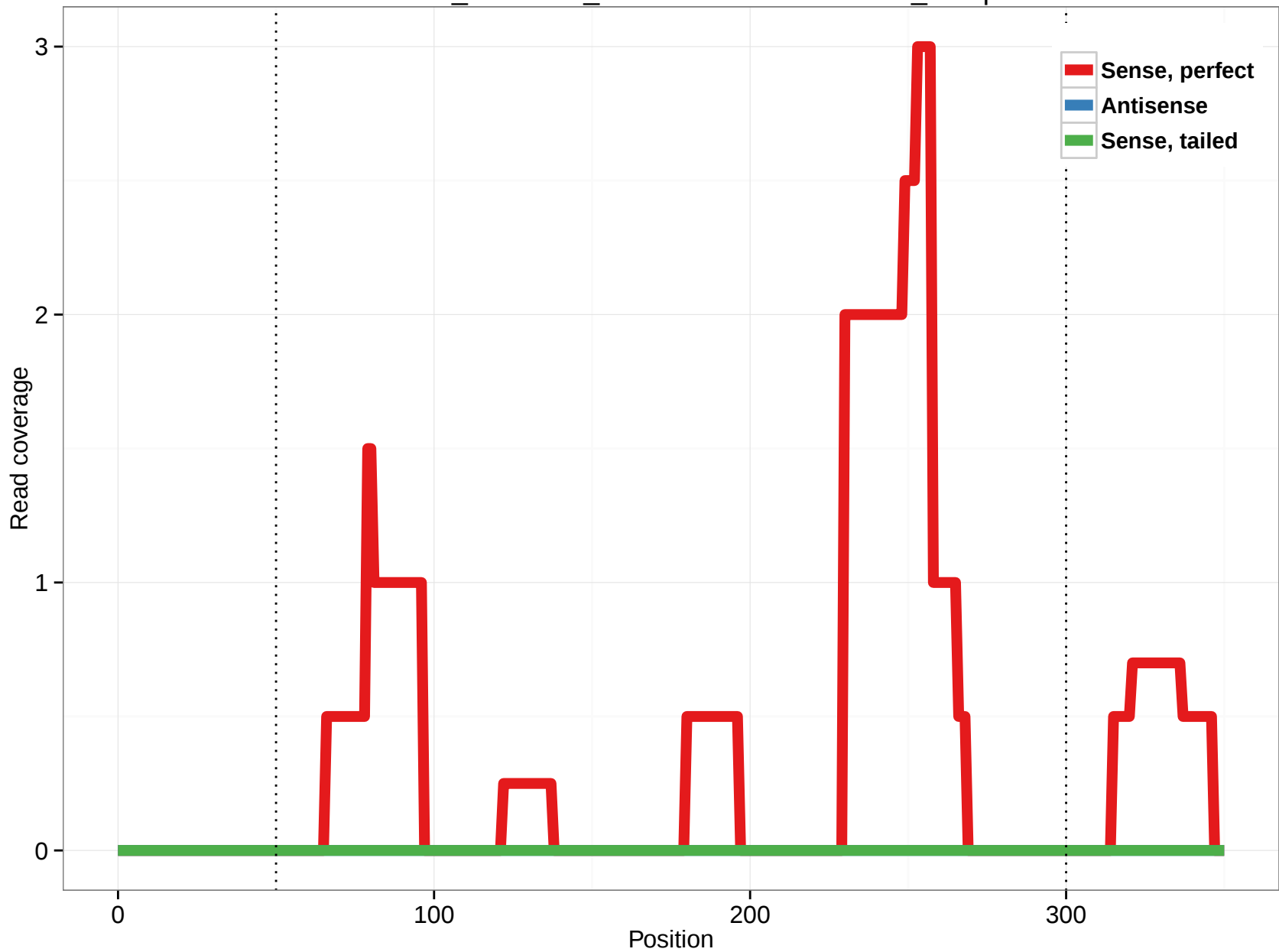
ornAna1_ensGene_ENSOANT00000024623_13.5p
