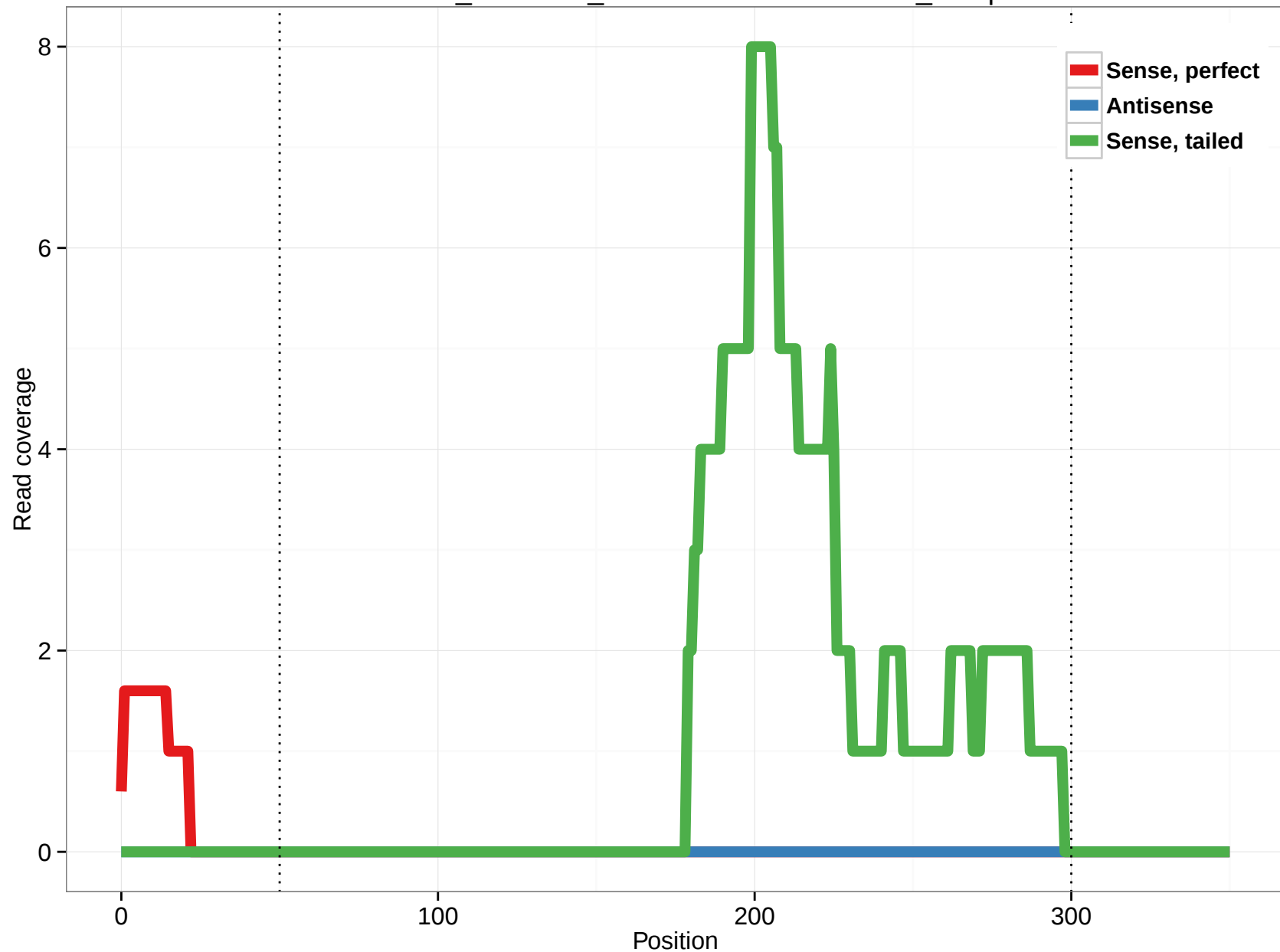
ornAna1_ensGene_ENSOANT00000024606_24.5p
