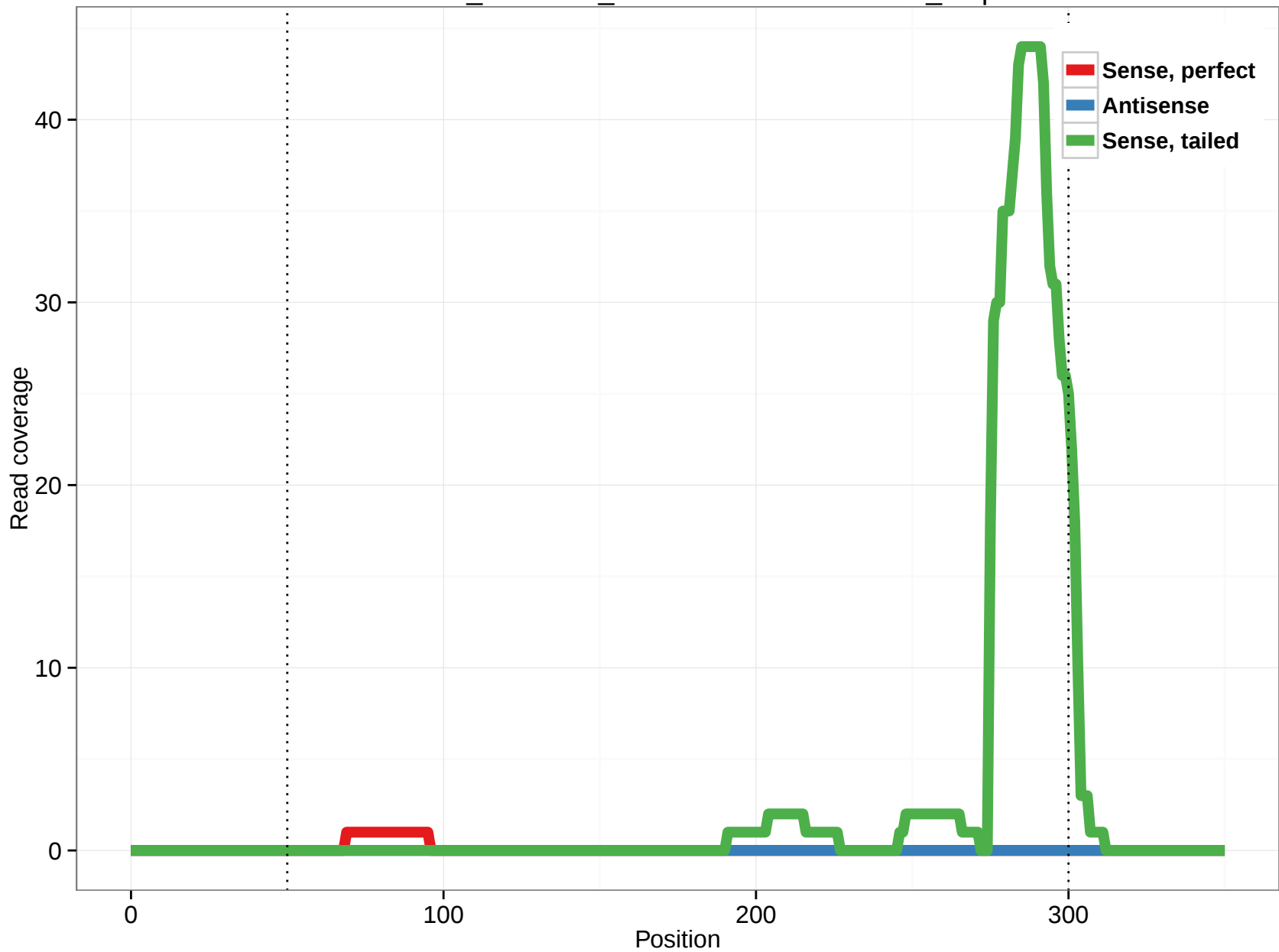
ornAna1_ensGene_ENSOANT00000024595_7.5p
