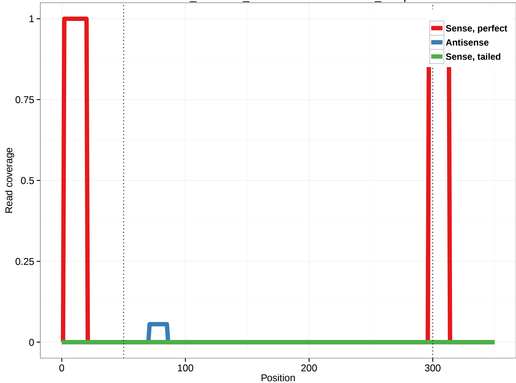
ornAna1_ensGene_ENSOANT00000024535_12.3p
