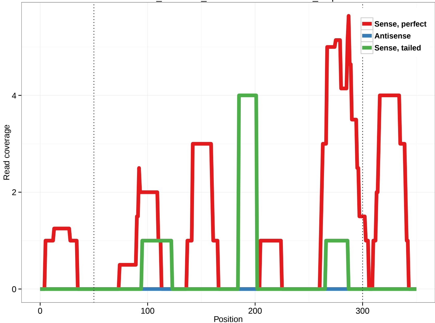
ornAna1_ensGene_ENSOANT00000024433_5.5p
