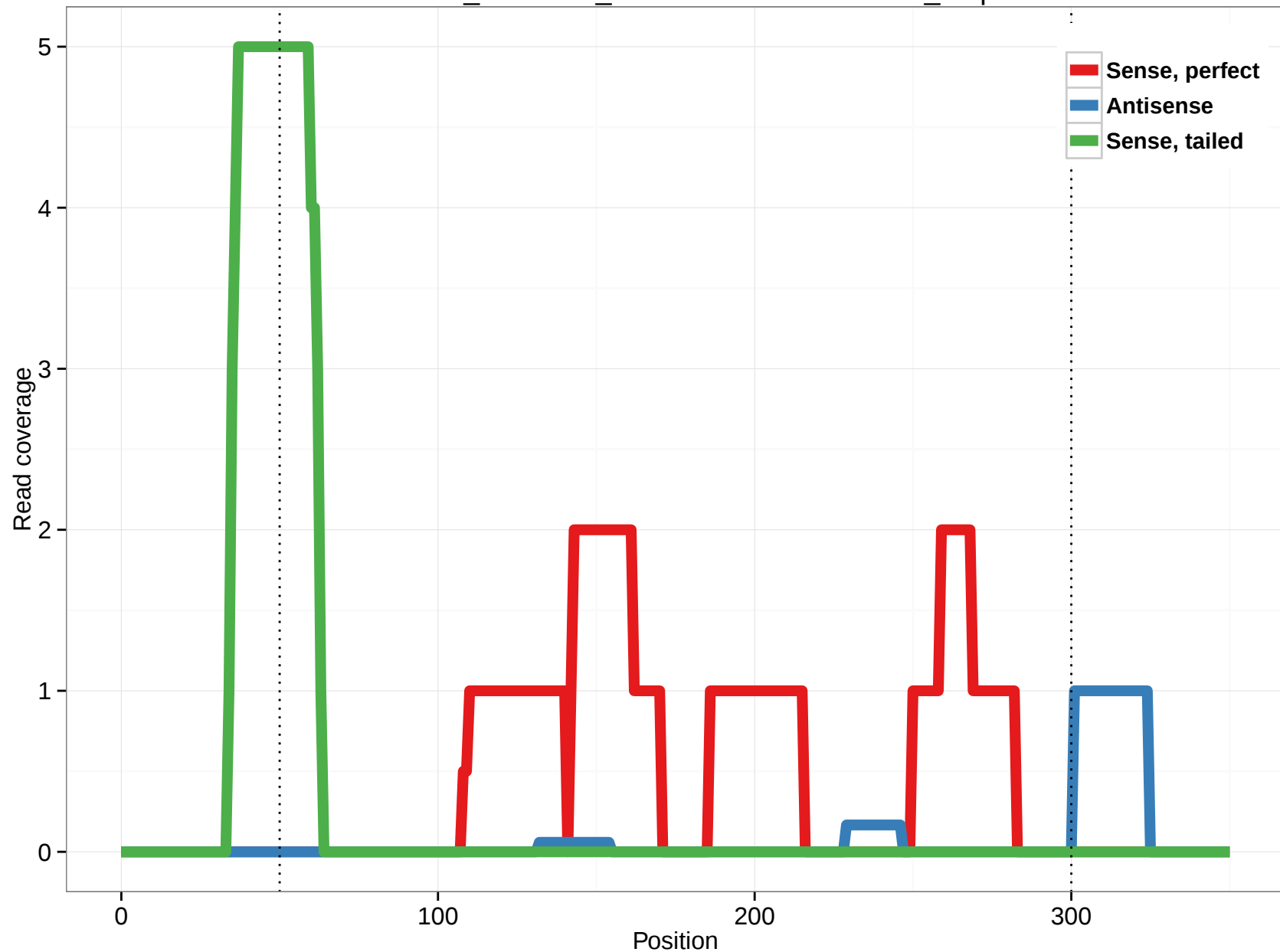
ornAna1_ensGene_ENSOANT00000024433_5.3p
