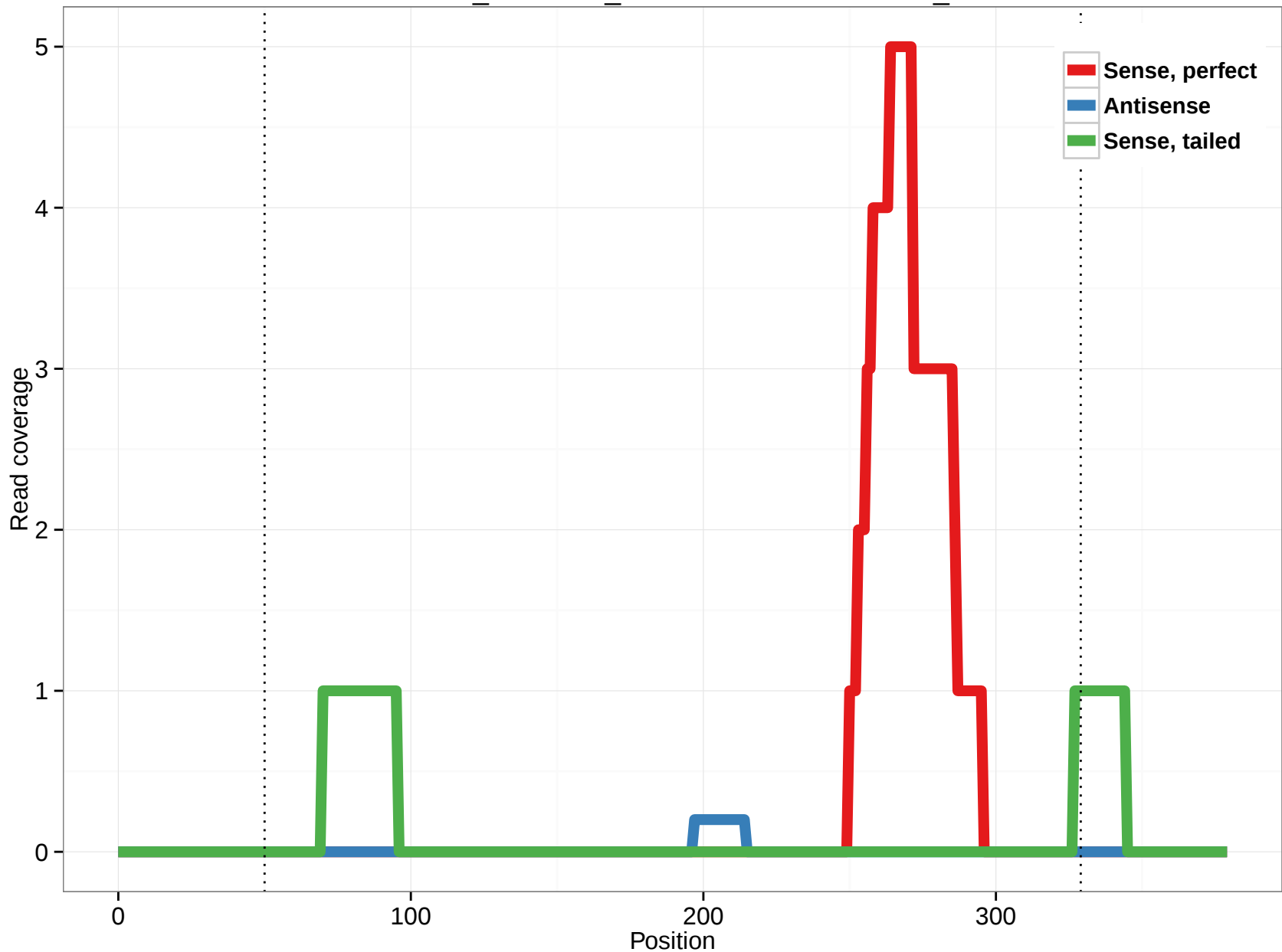
ornAna1_ensGene_ENSOANT00000024308_13
