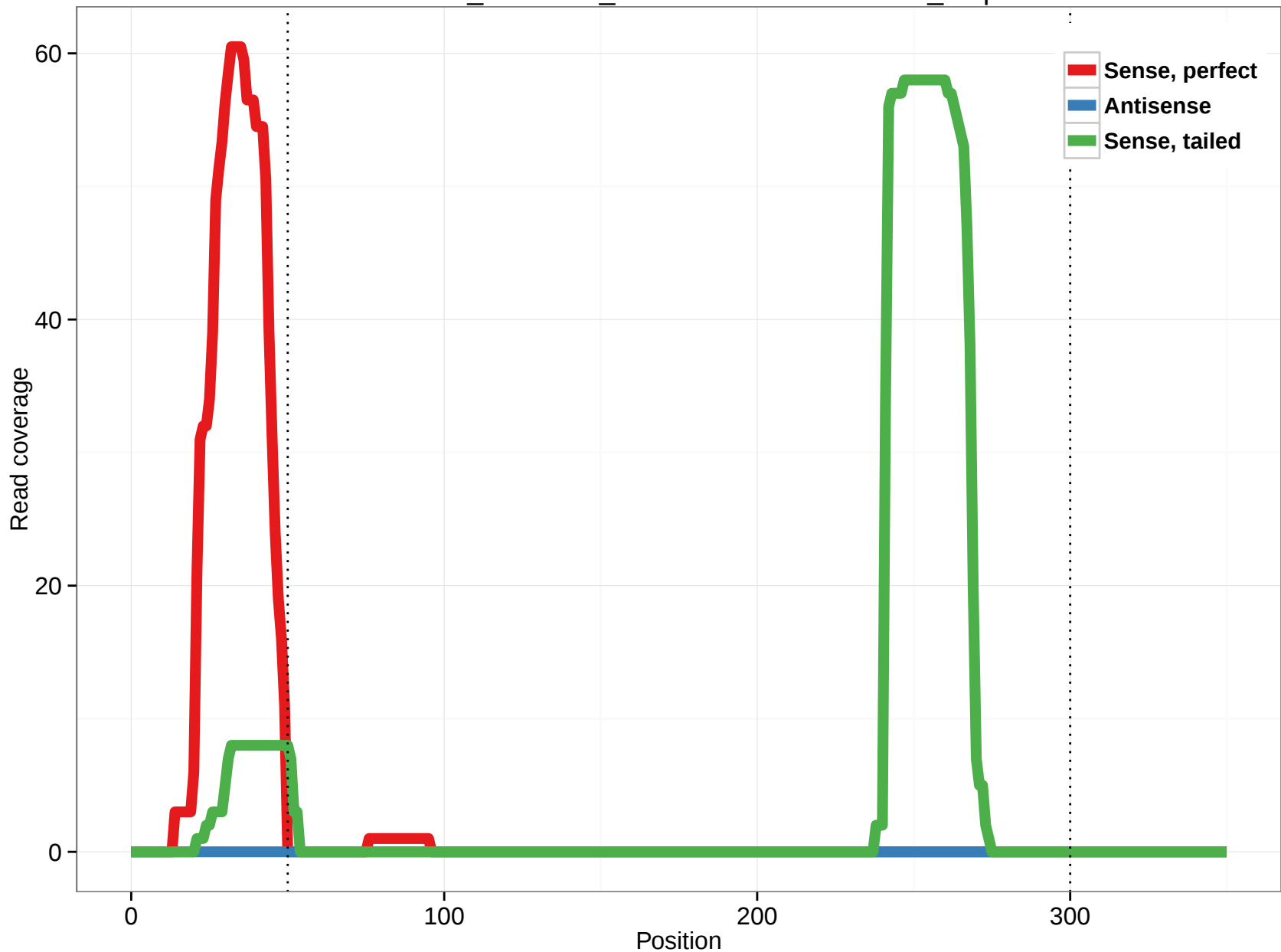
ornAna1_ensGene_ENSOANT00000024303_1.5p
