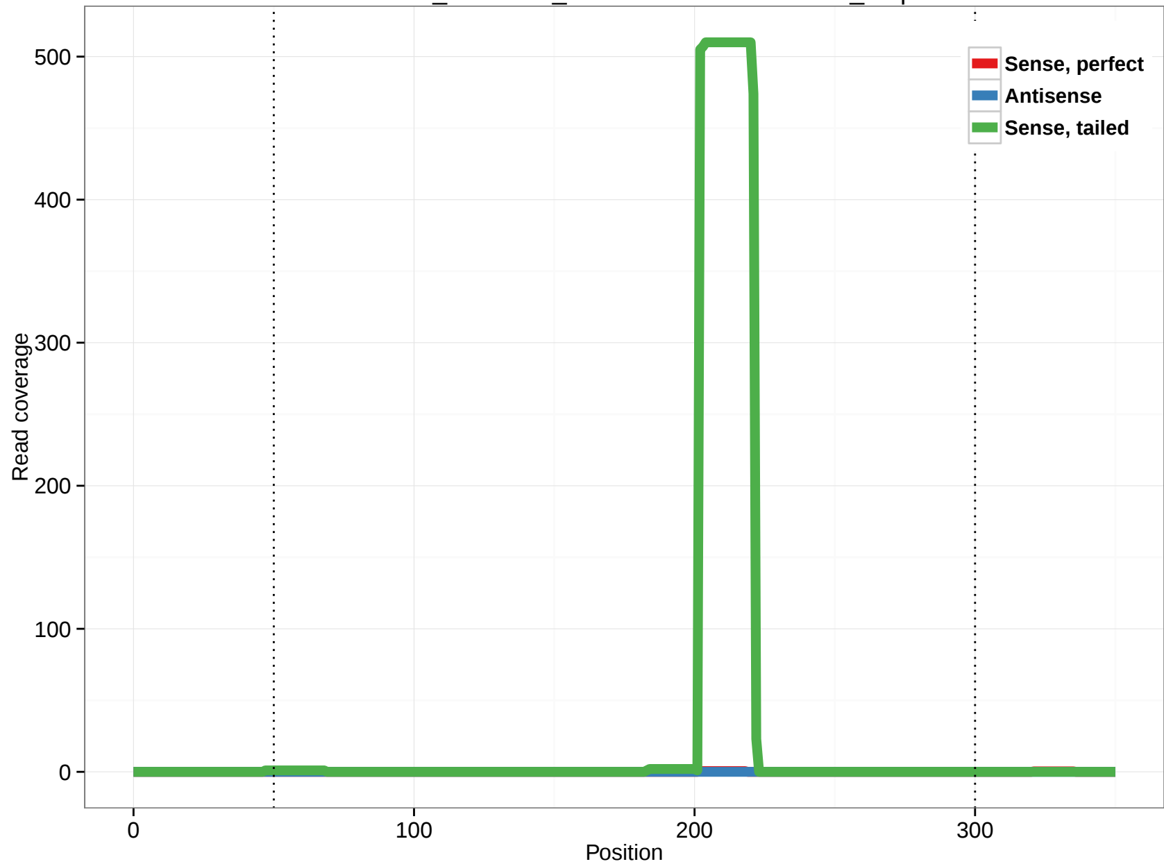
ornAna1_ensGene_ENSOANT00000024175_5.3p
