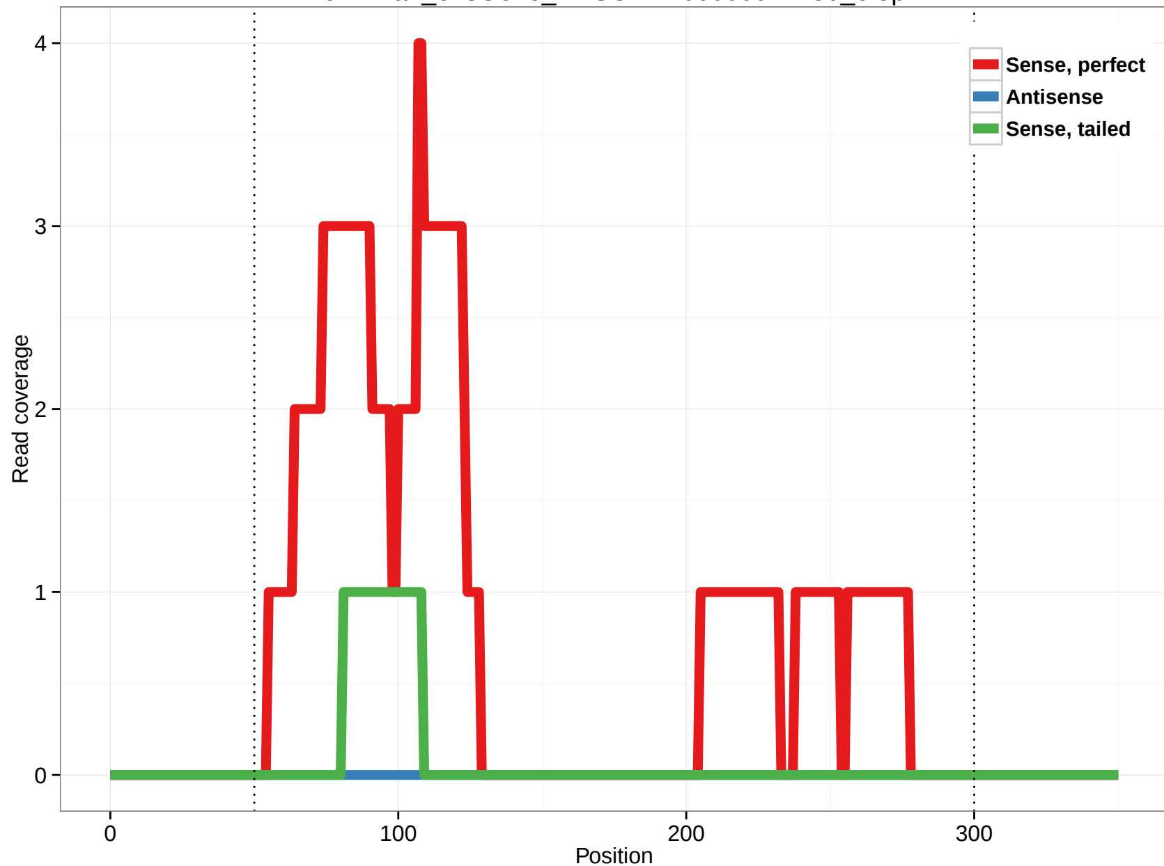
ornAna1_ensGene_ENSOANT00000024150_6.5p
