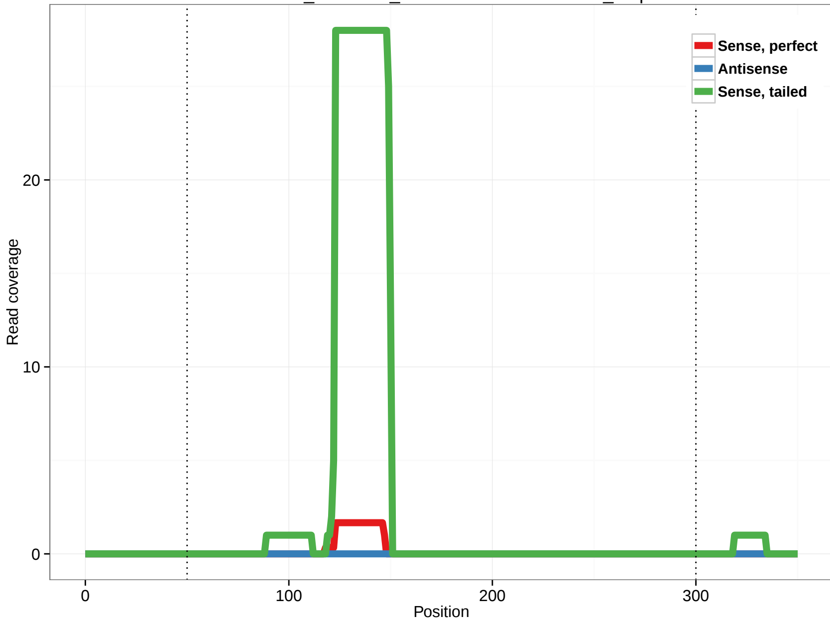
ornAna1_ensGene_ENSOANT00000024129_3.3p
