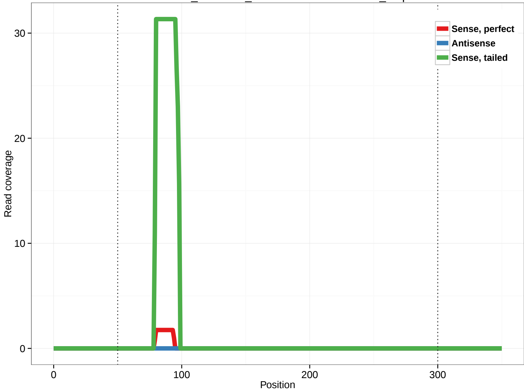
ornAna1_ensGene_ENSOANT00000024102_7.5p
