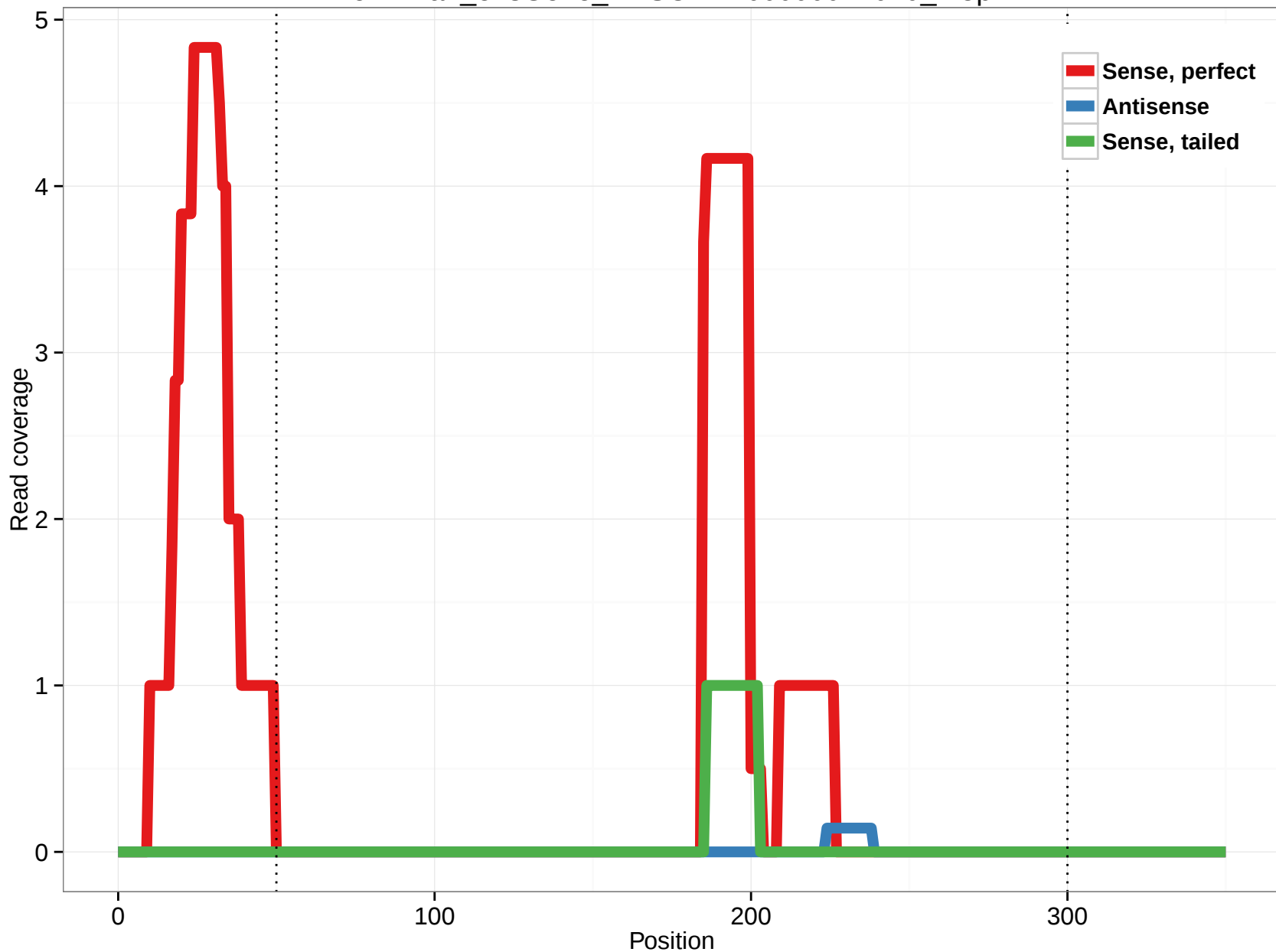
ornAna1_ensGene_ENSOANT00000024070_2.5p
