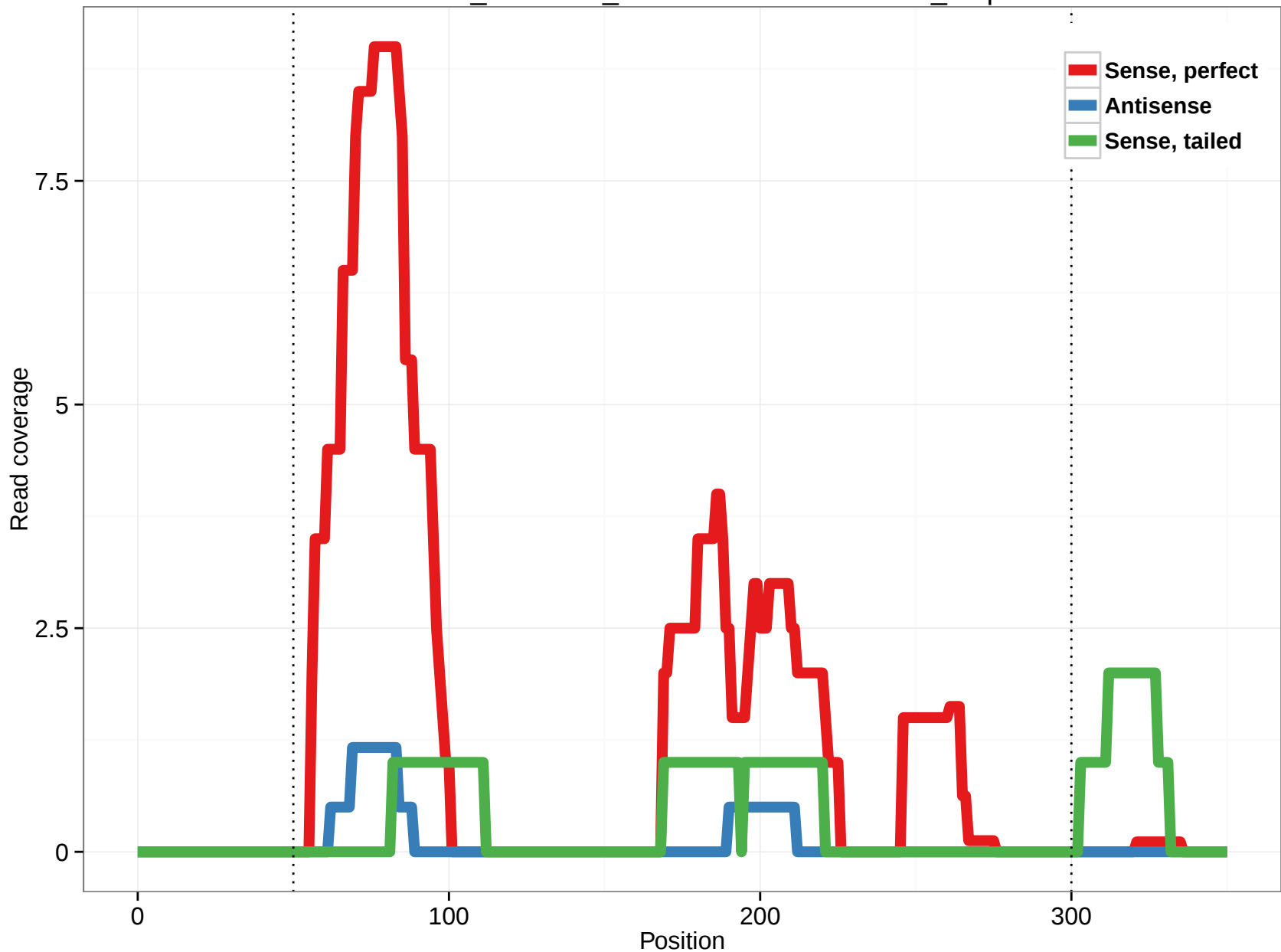
ornAna1_ensGene_ENSOANT00000024039_7.5p
