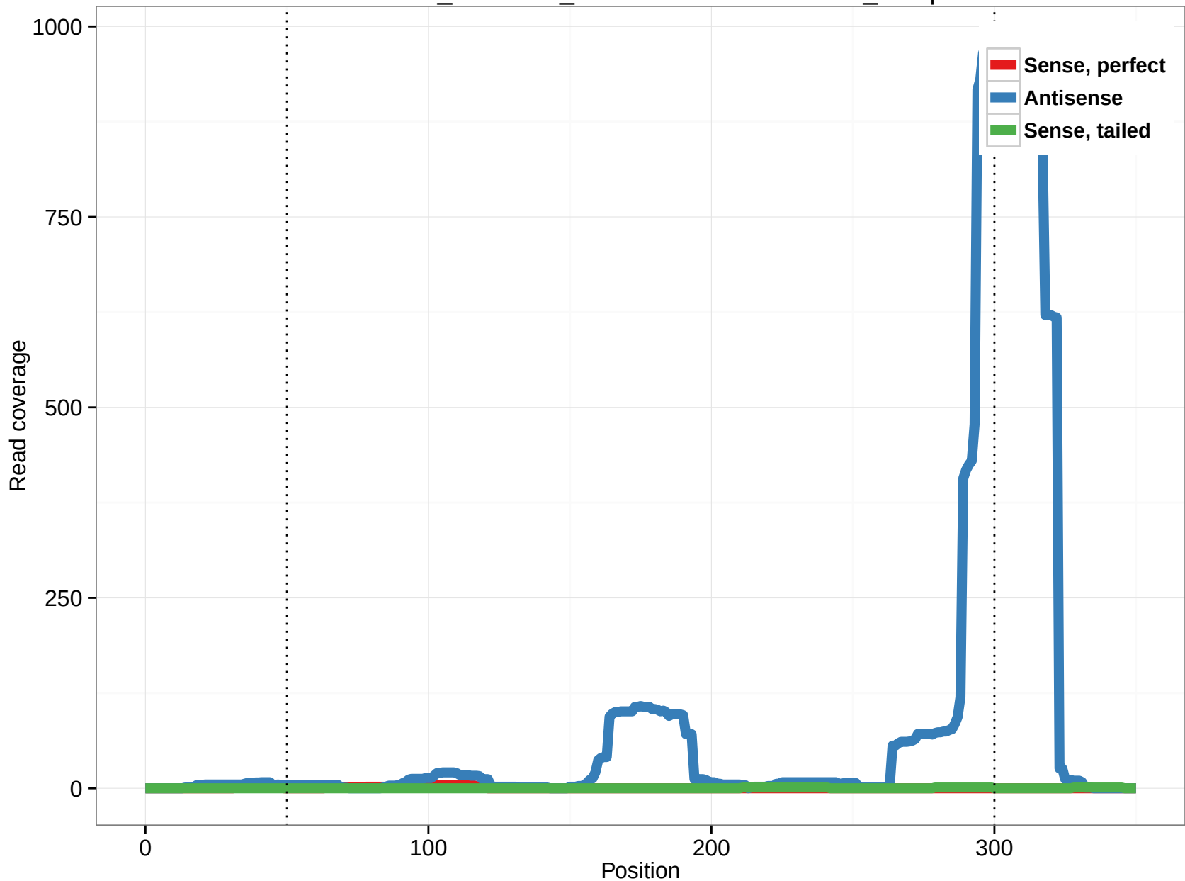
ornAna1_ensGene_ENSOANT00000024039_14.3p
