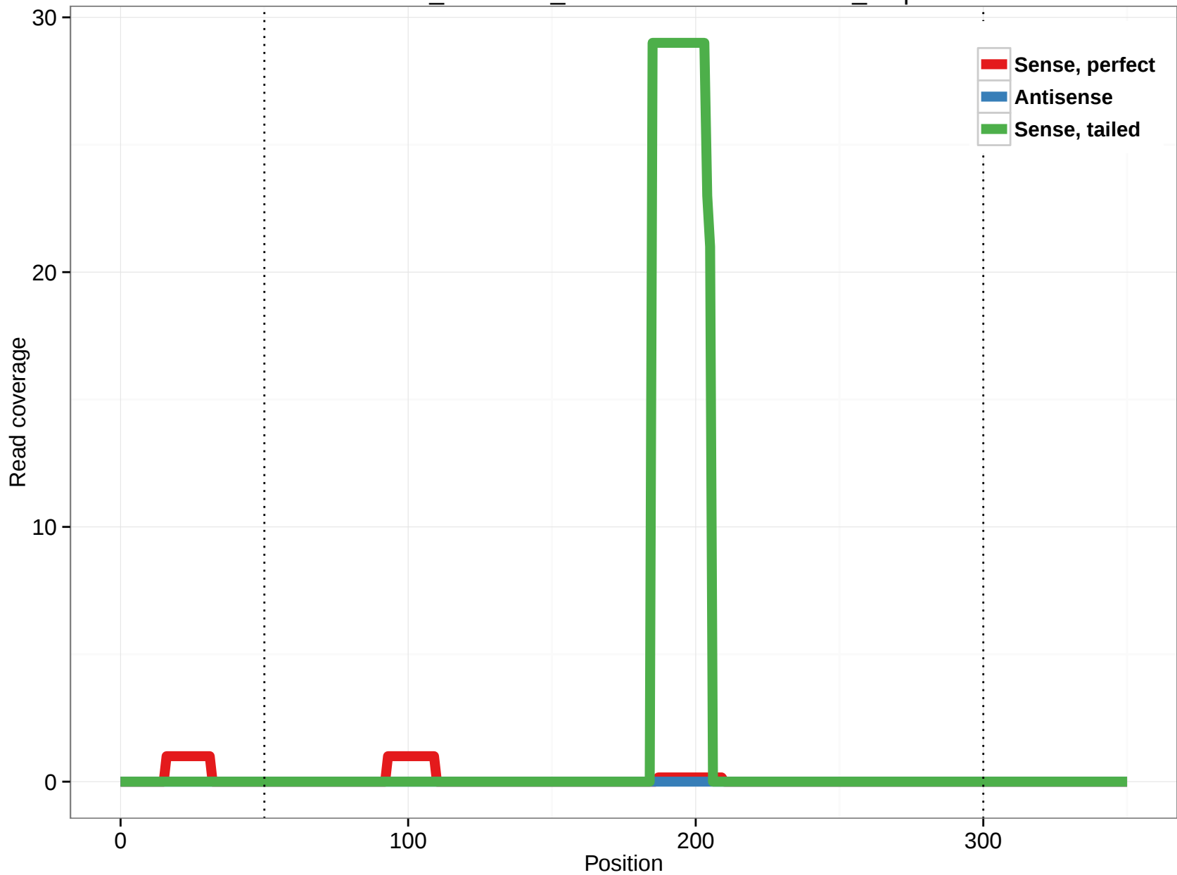
ornAna1_ensGene_ENSOANT00000023953_2.5p
