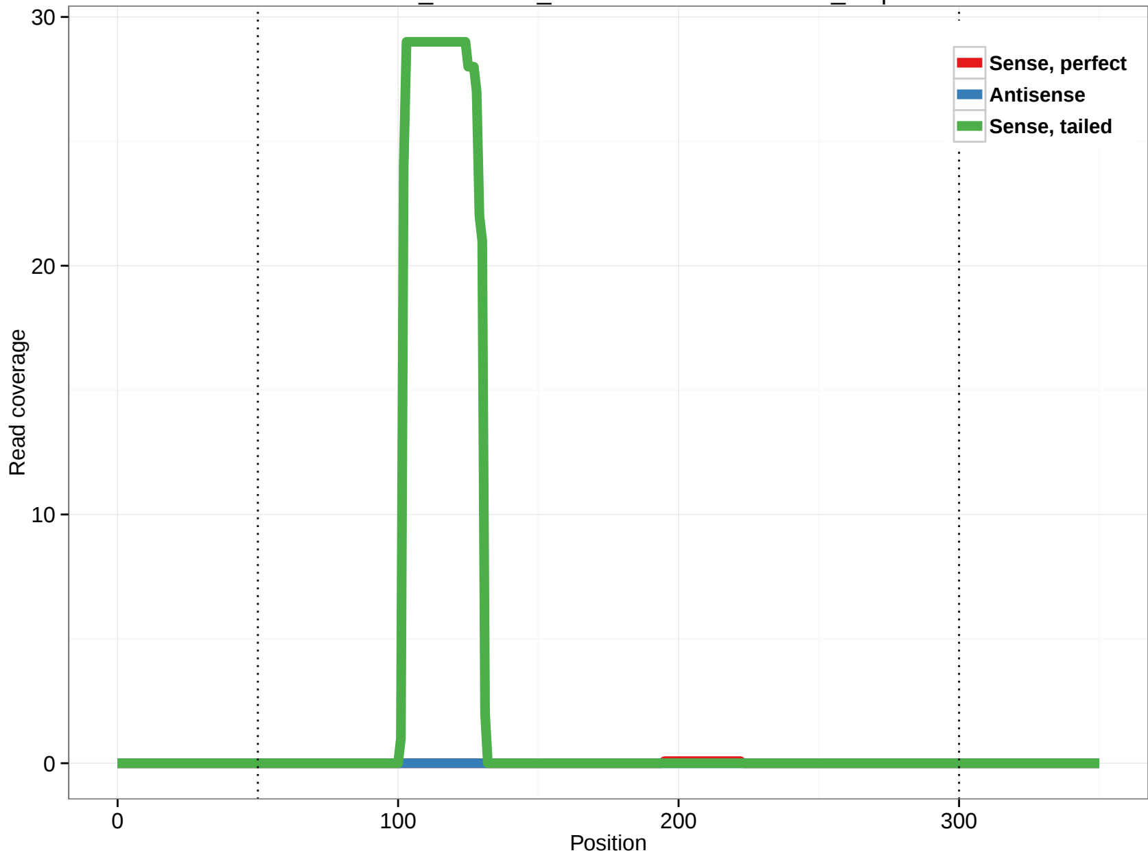
ornAna1_ensGene_ENSOANT00000023895_6.5p
