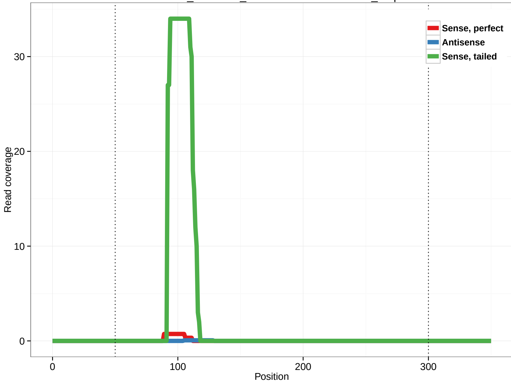
ornAna1_ensGene_ENSOANT00000023853_1.5p
