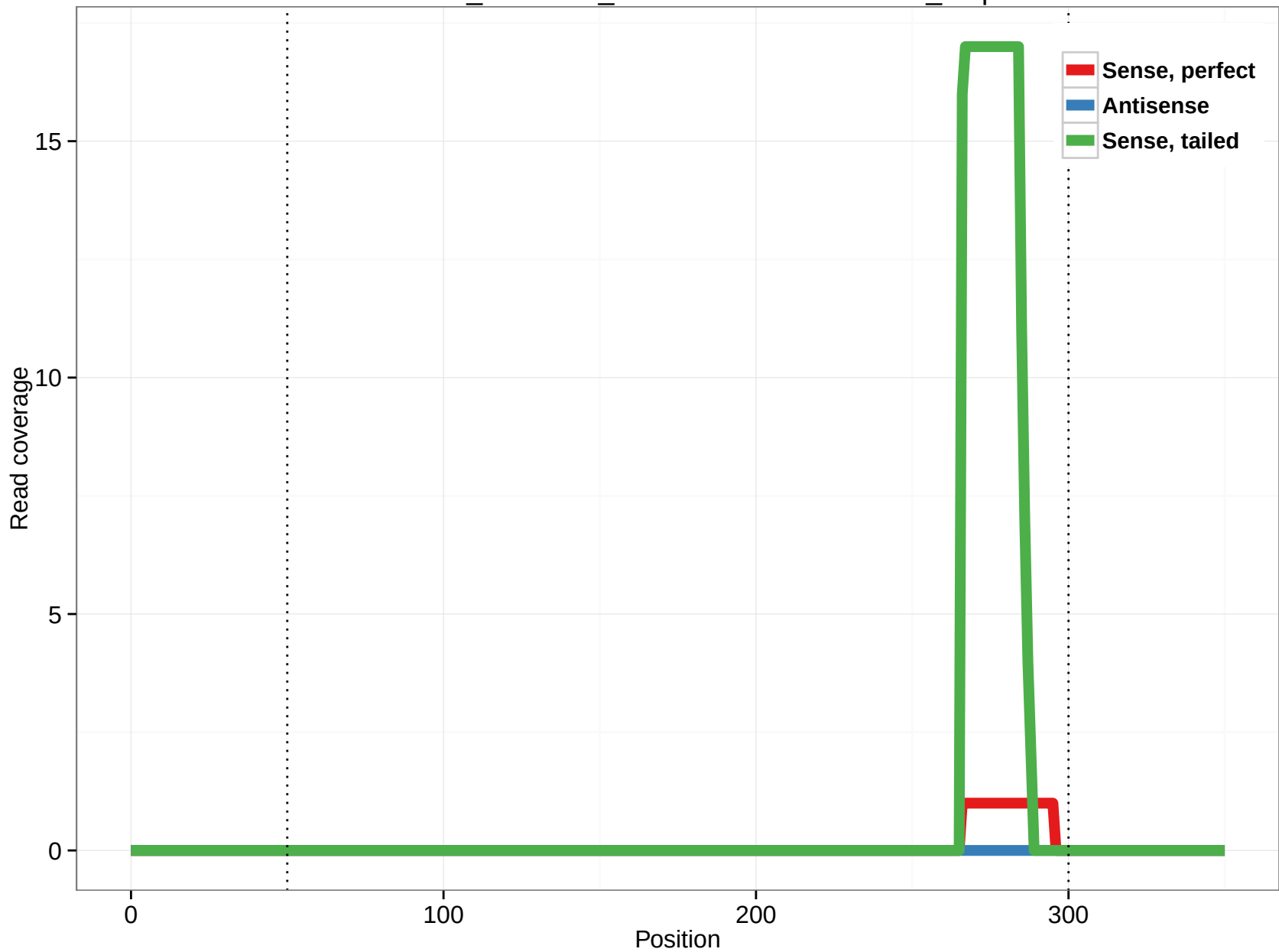
ornAna1_ensGene_ENSOANT00000023825_0.5p
