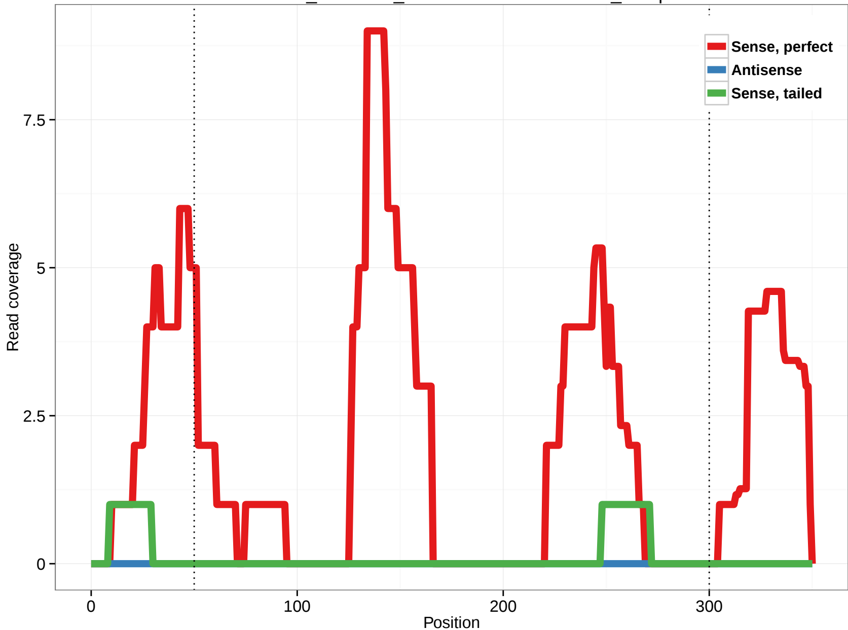
ornAna1_ensGene_ENSOANT00000023808_11.5p
