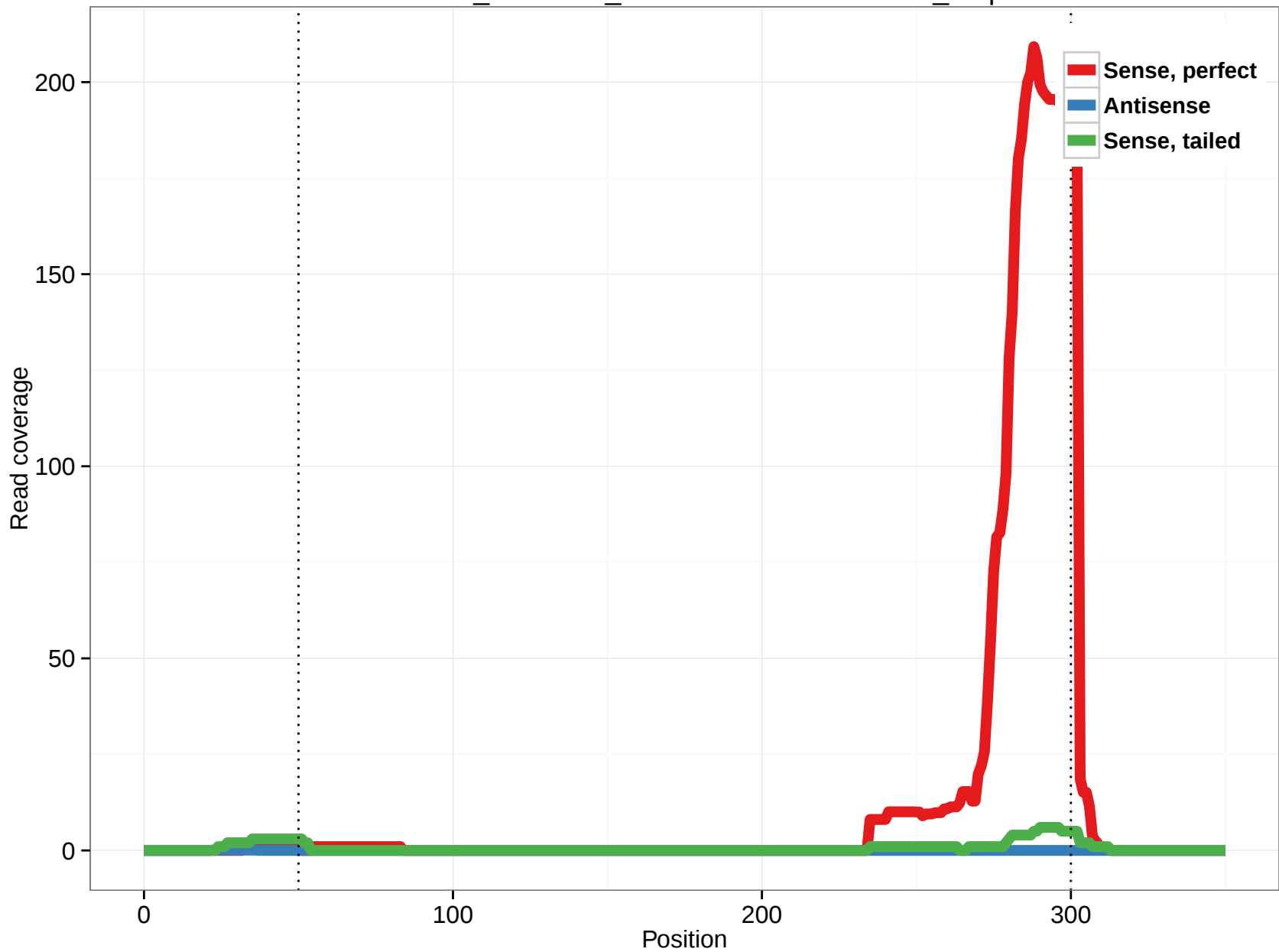
ornAna1_ensGene_ENSOANT00000023550_2.5p
