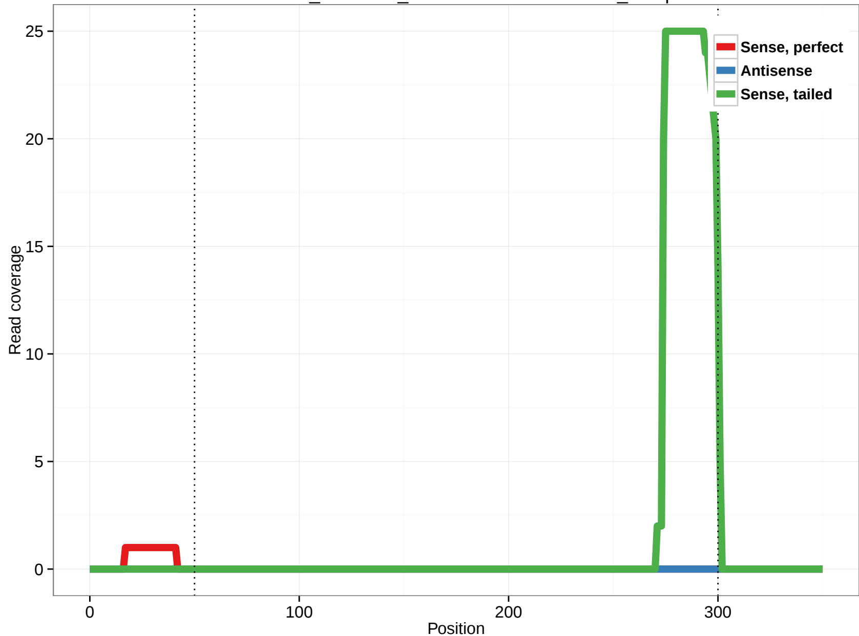
ornAna1_ensGene_ENSOANT00000023508_16.5p
