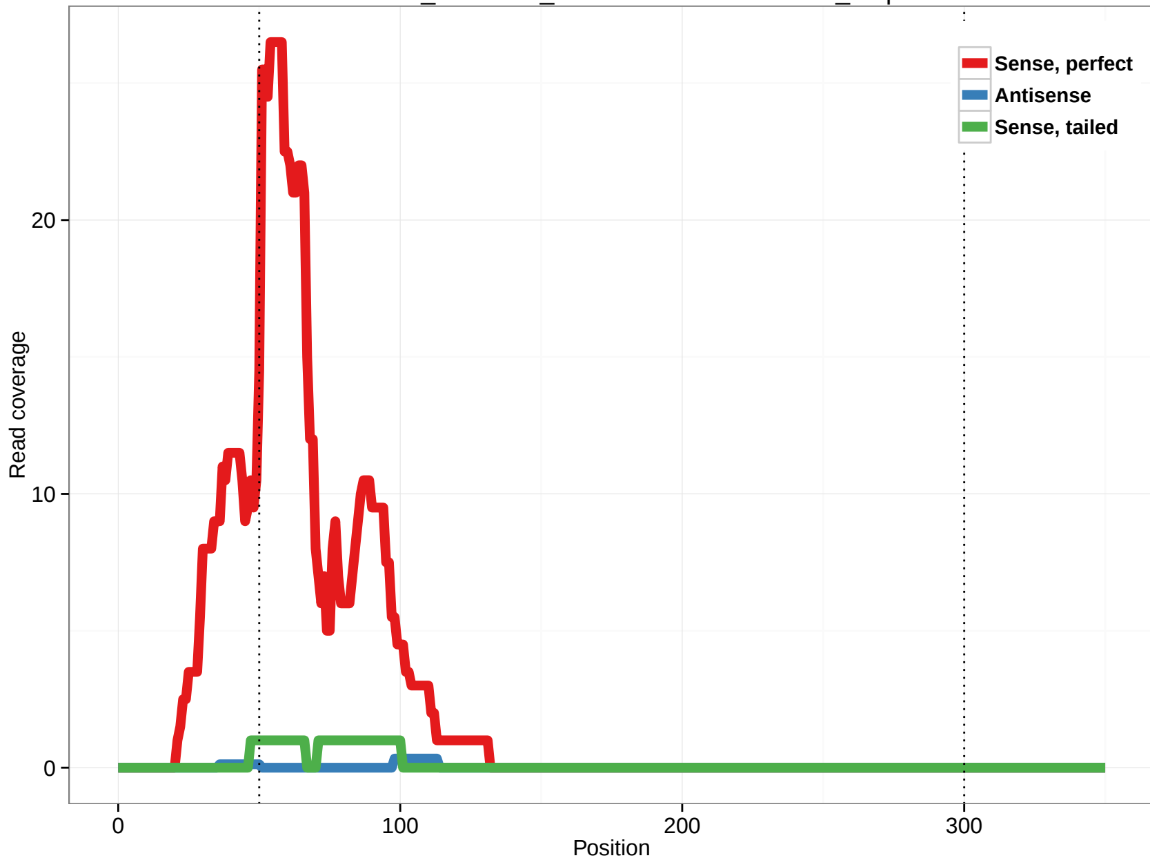
ornAna1_ensGene_ENSOANT00000023469_0.5p
