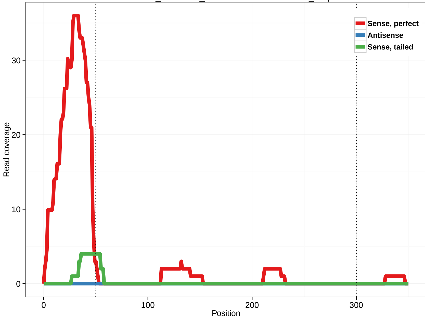
ornAna1_ensGene_ENSOANT00000023446_1.5p
