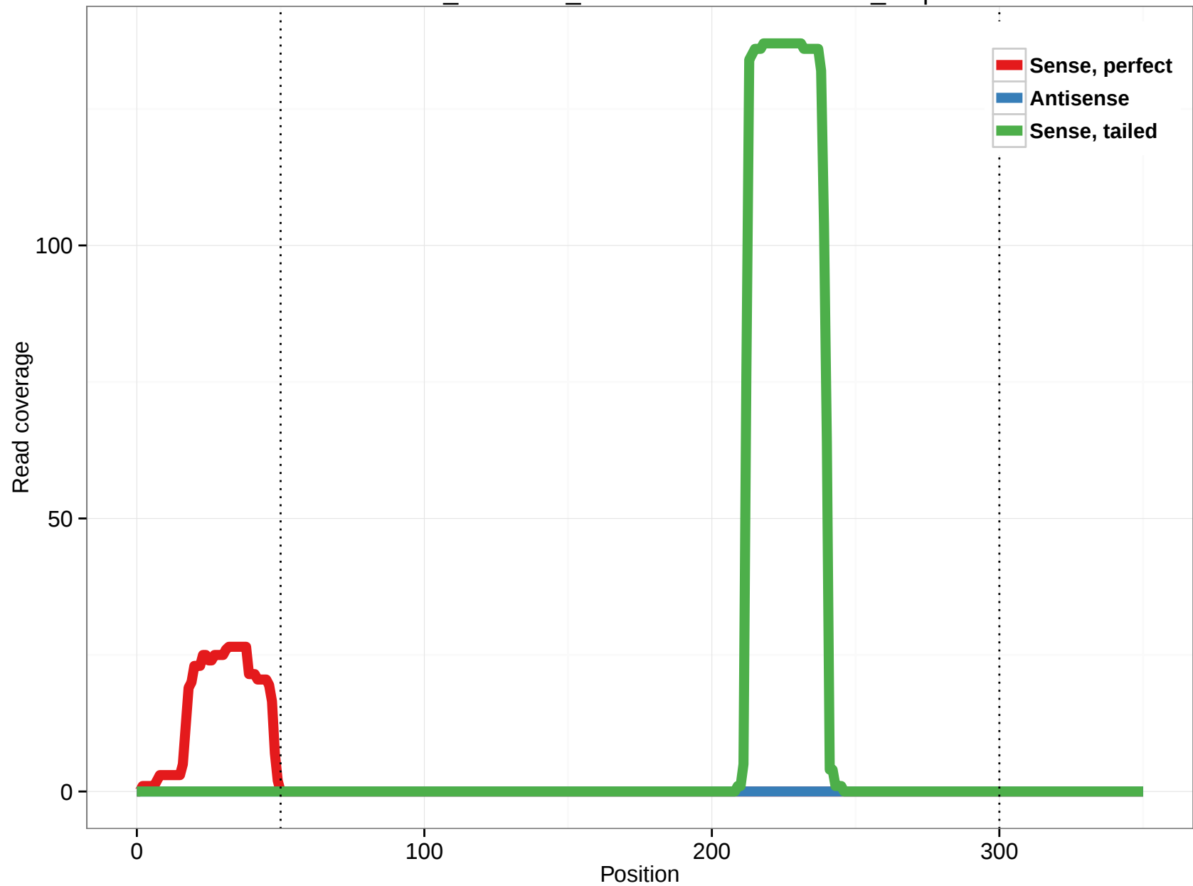
ornAna1_ensGene_ENSOANT00000023446_0.5p
