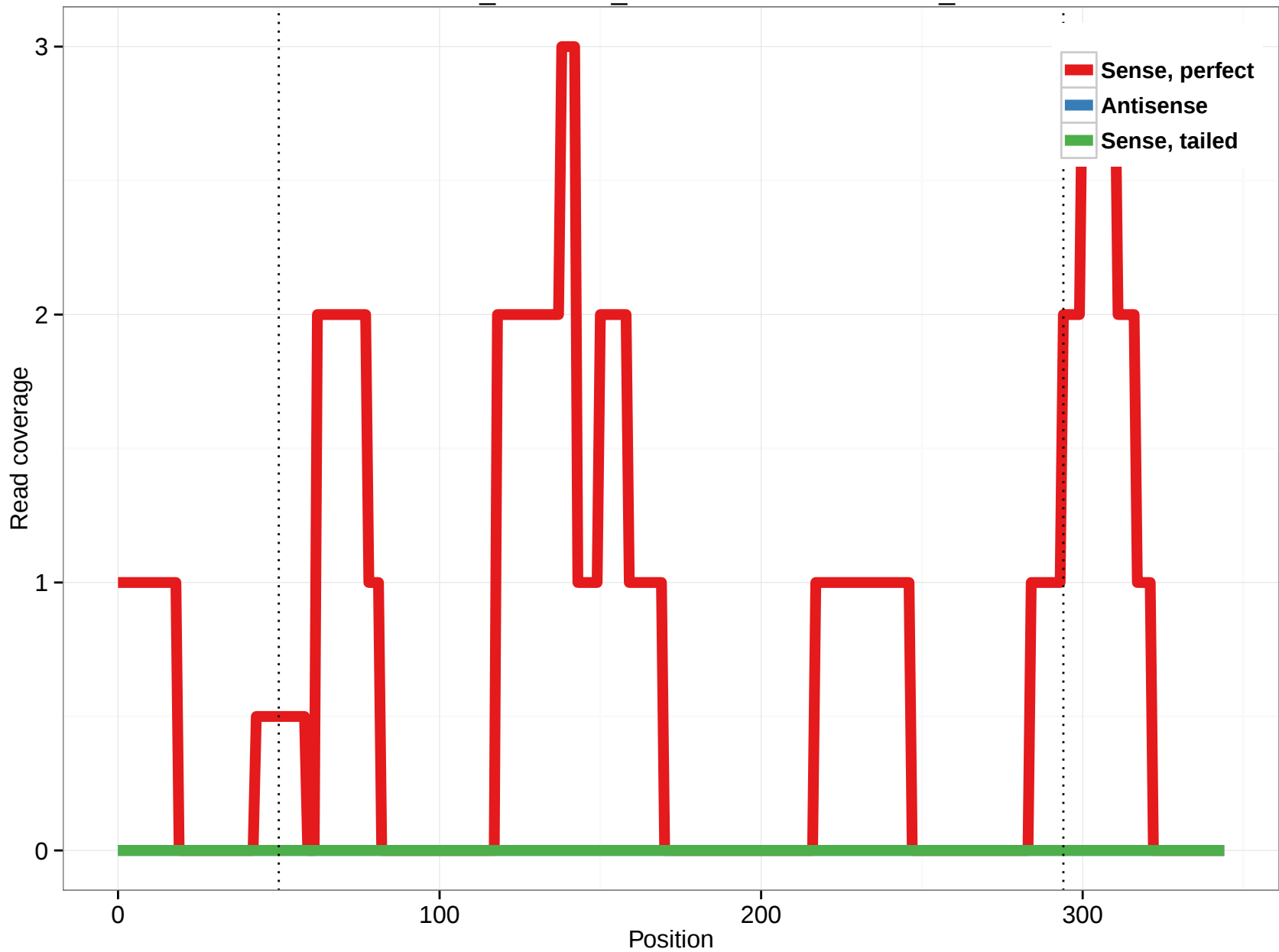
ornAna1_ensGene_ENSOANT00000023398_3
