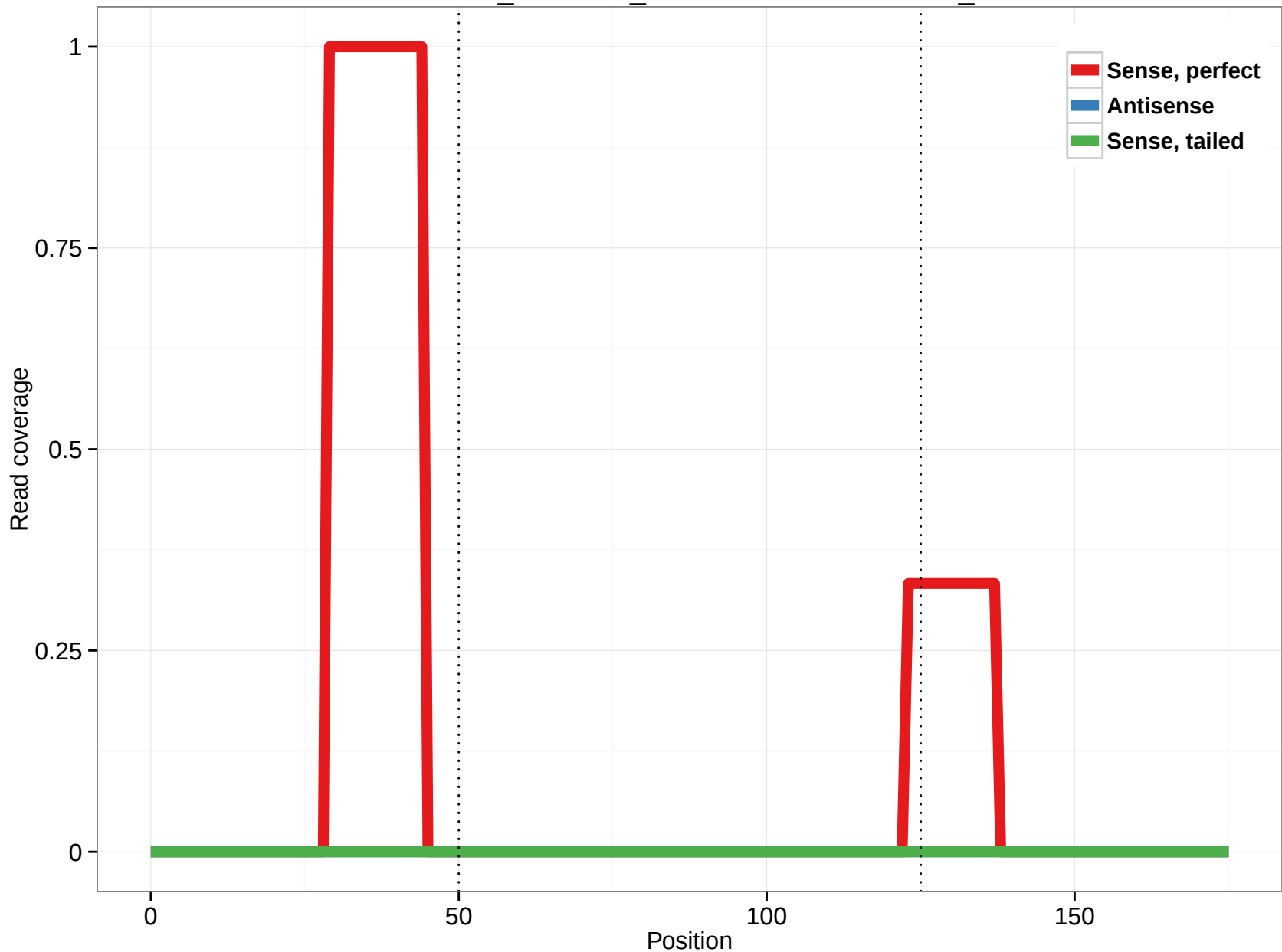
ornAna1_ensGene_ENSOANT00000023336_2
