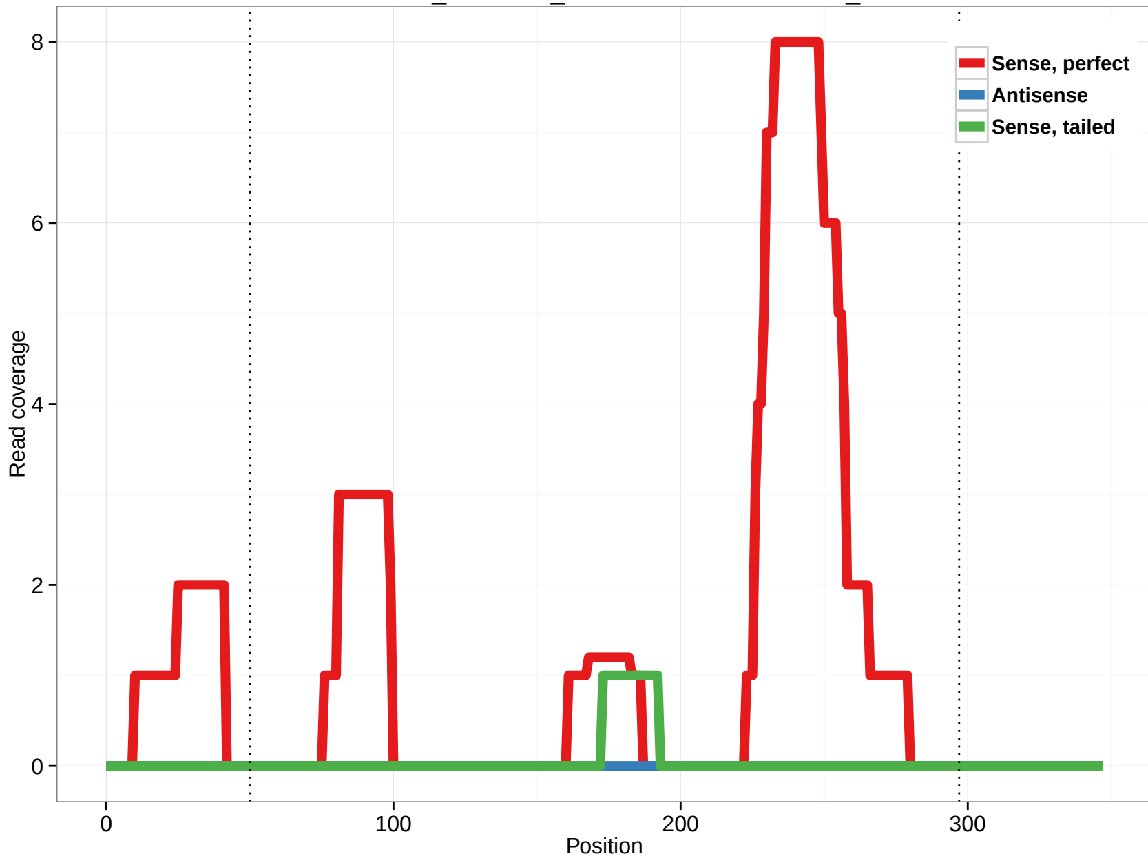
ornAna1_ensGene_ENSOANT00000023329_1
