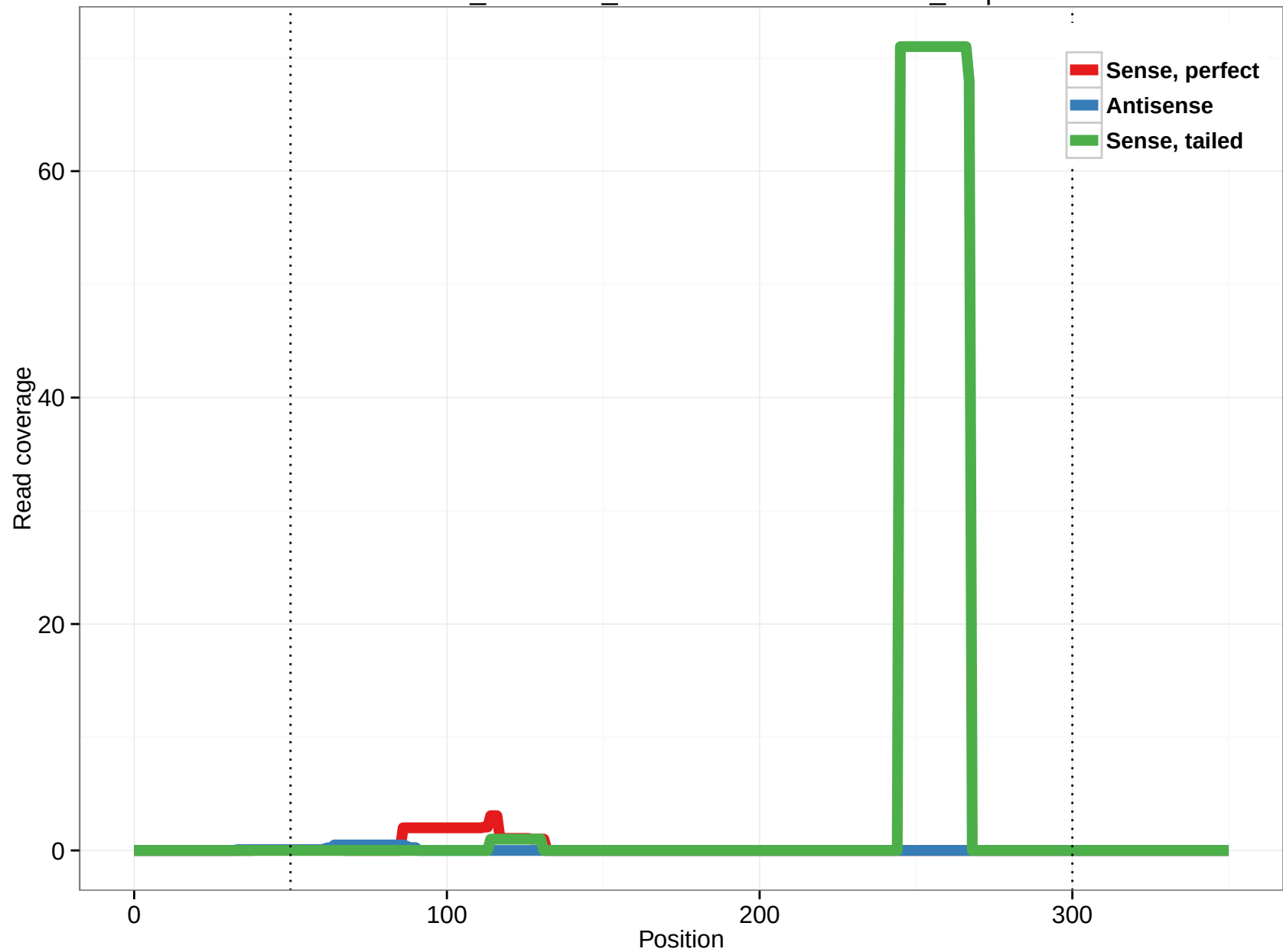
ornAna1_ensGene_ENSOANT00000023301_0.3p
