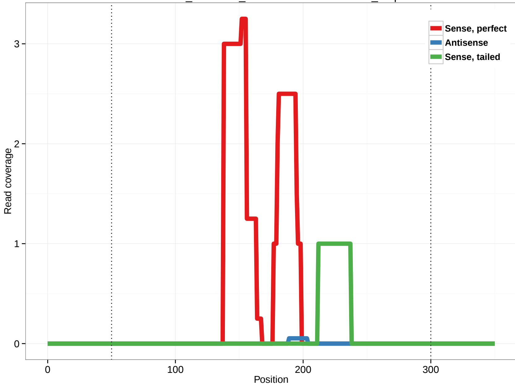
ornAna1_ensGene_ENSOANT00000023276_1.5p
