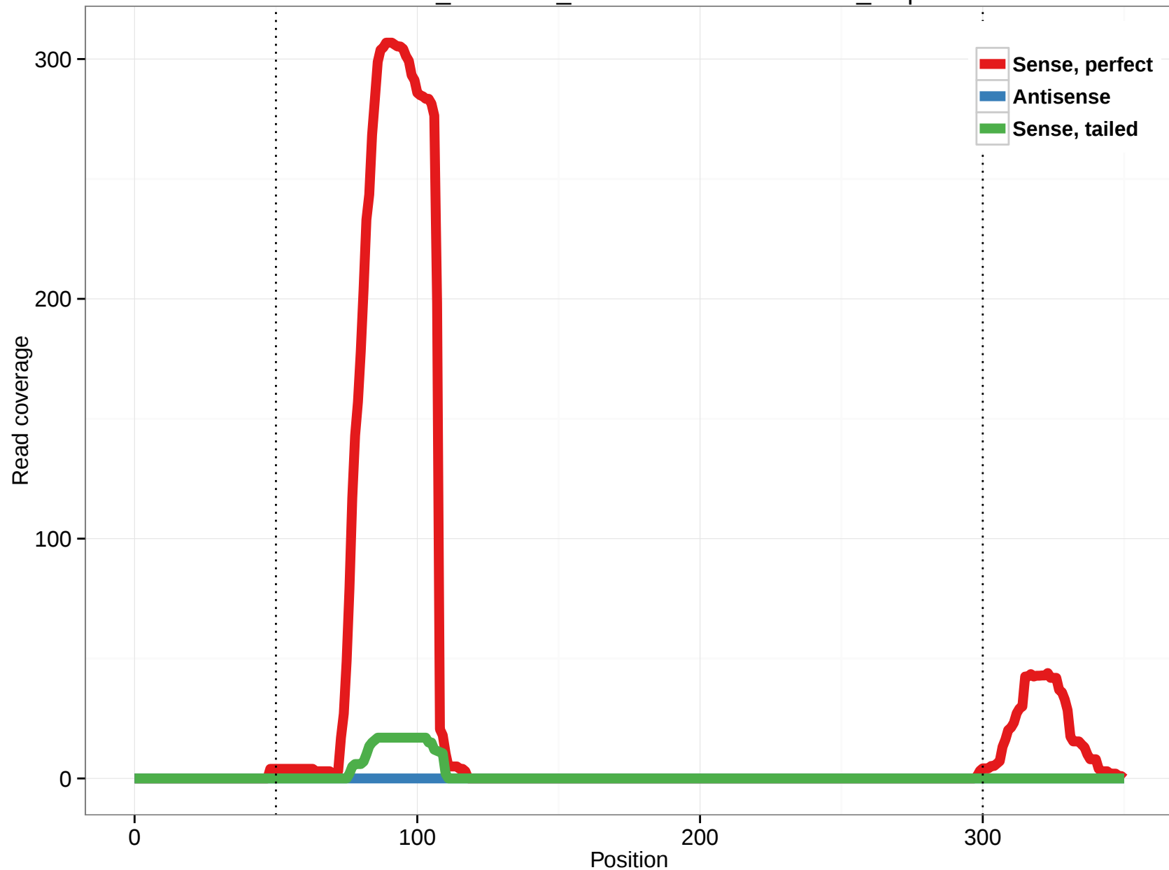
ornAna1_ensGene_ENSOANT00000023245_0.3p
