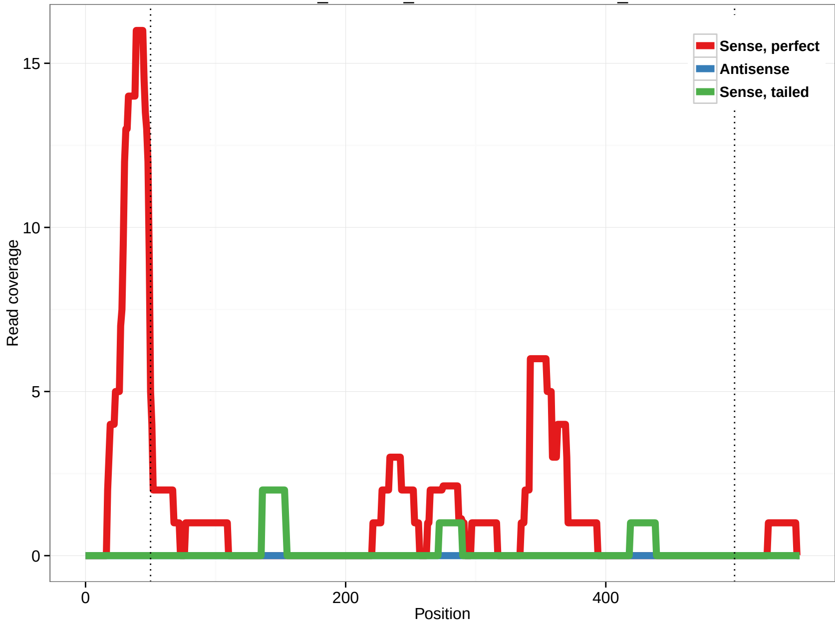
ornAna1_ensGene_ENSOANT00000023220_1
