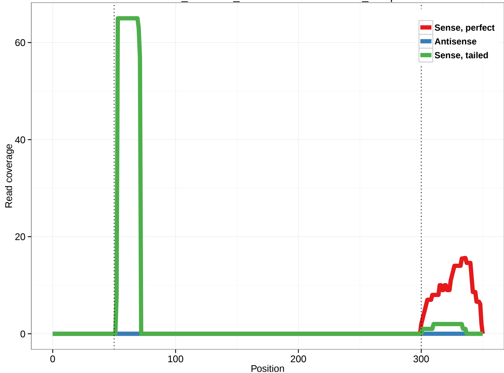
ornAna1_ensGene_ENSOANT00000023126_14.3p
