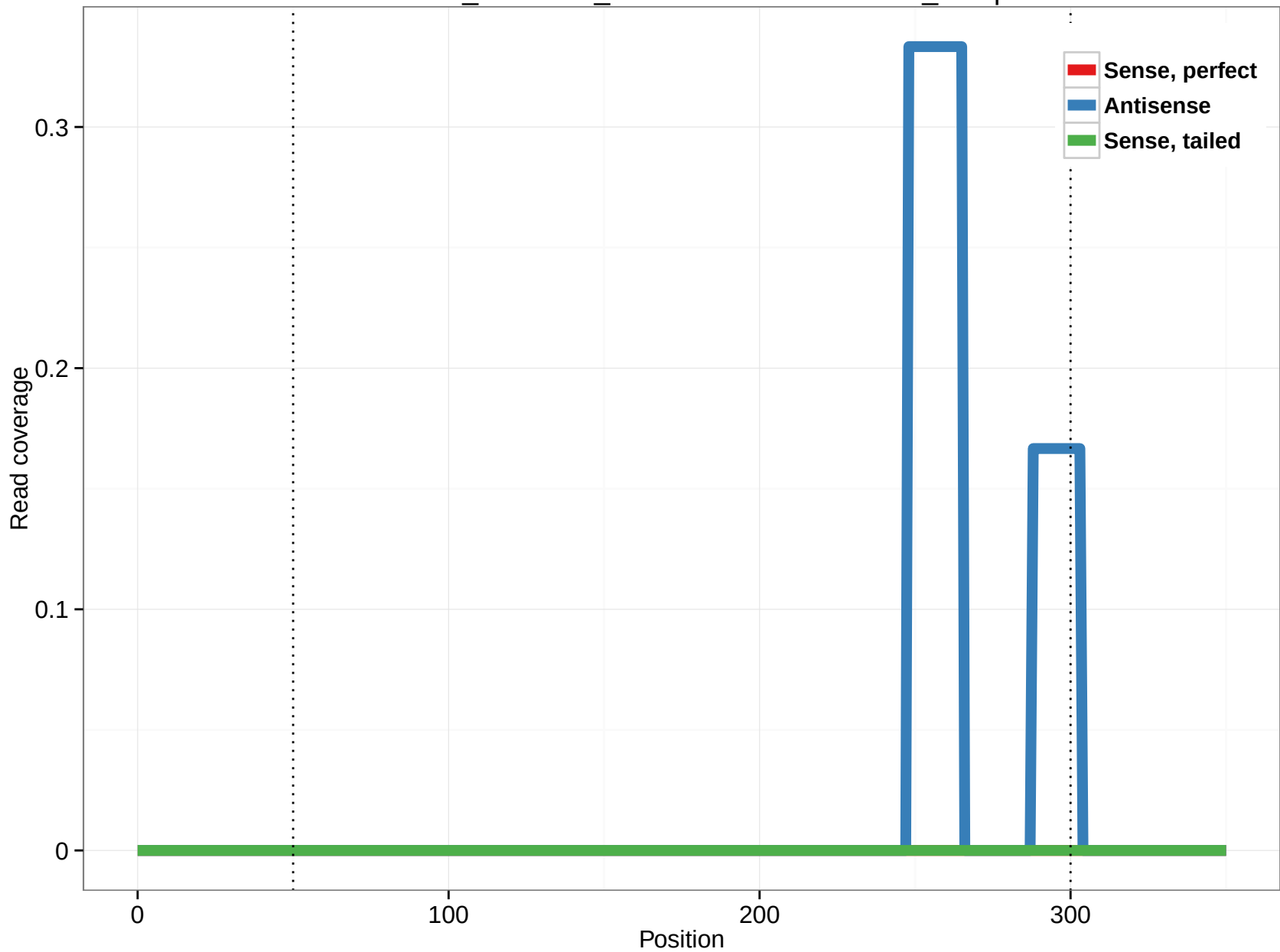
ornAna1_ensGene_ENSOANT00000023109_15.3p
