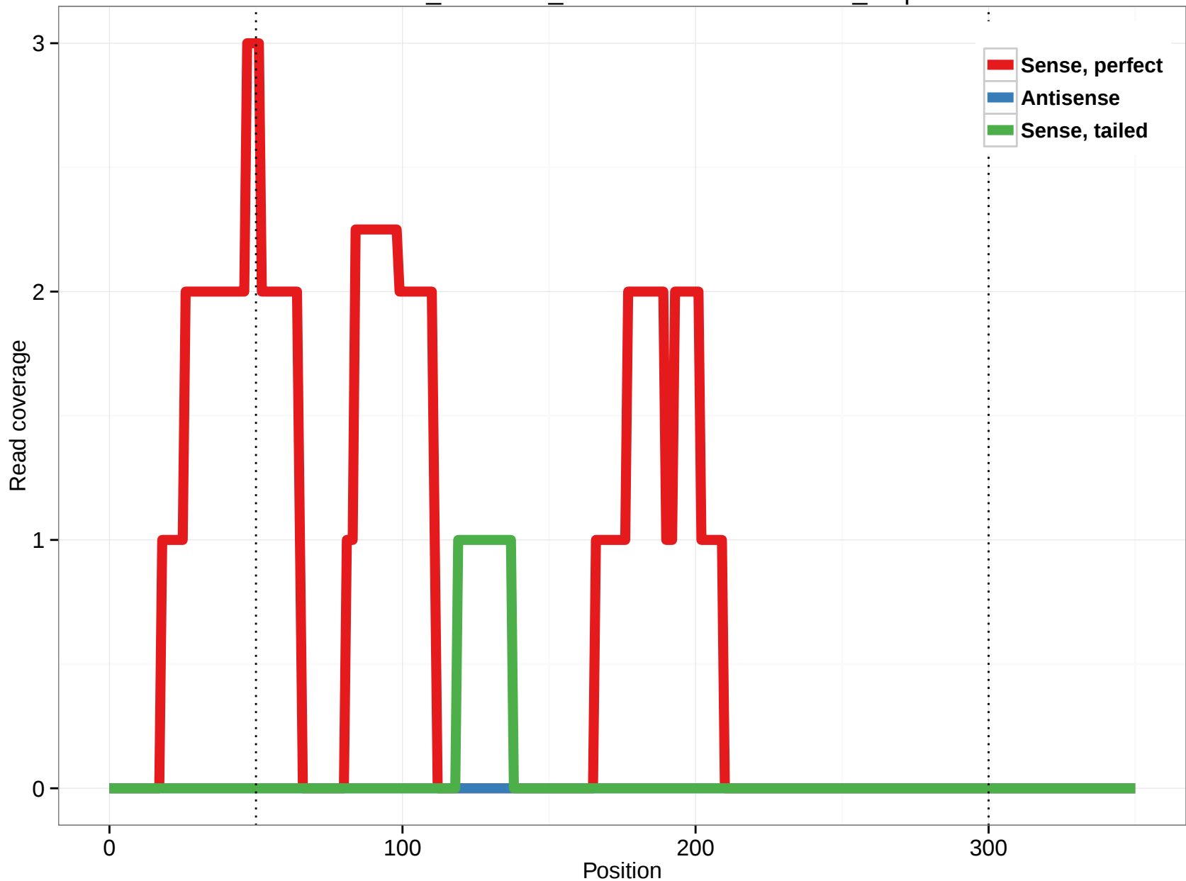
ornAna1_ensGene_ENSOANT00000023079_7.5p
